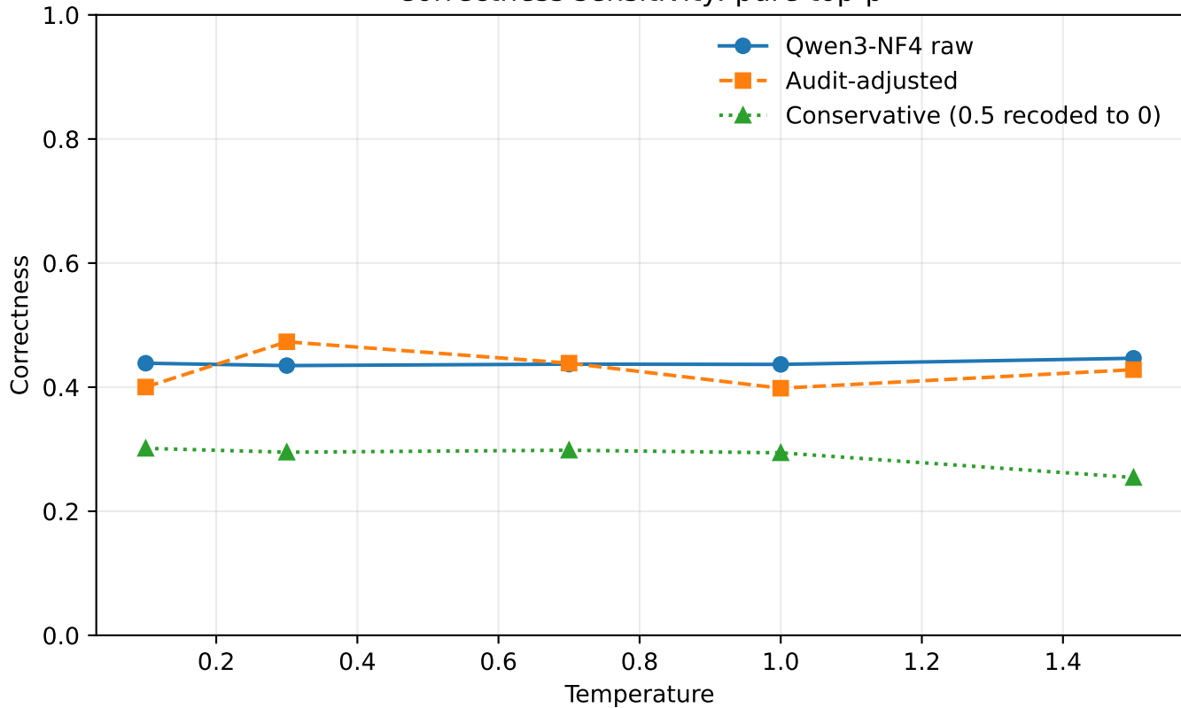
Correctness sensitivity: pure top-p
