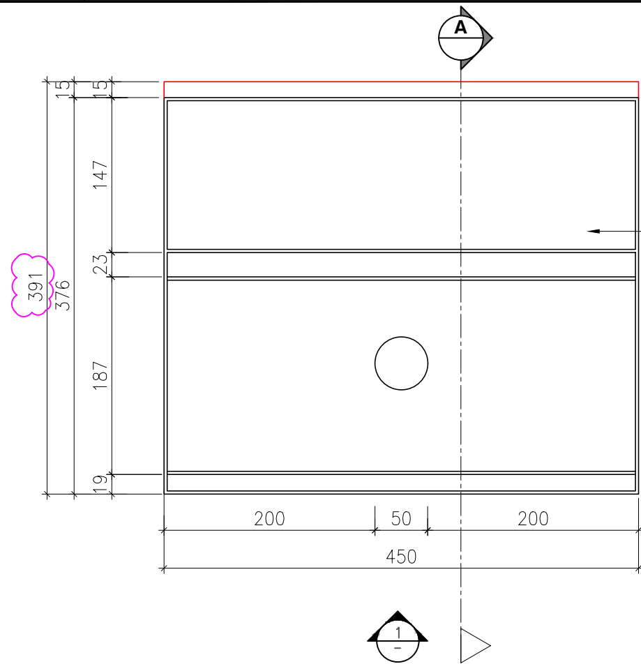
1 PLAN SCALE 1:5
