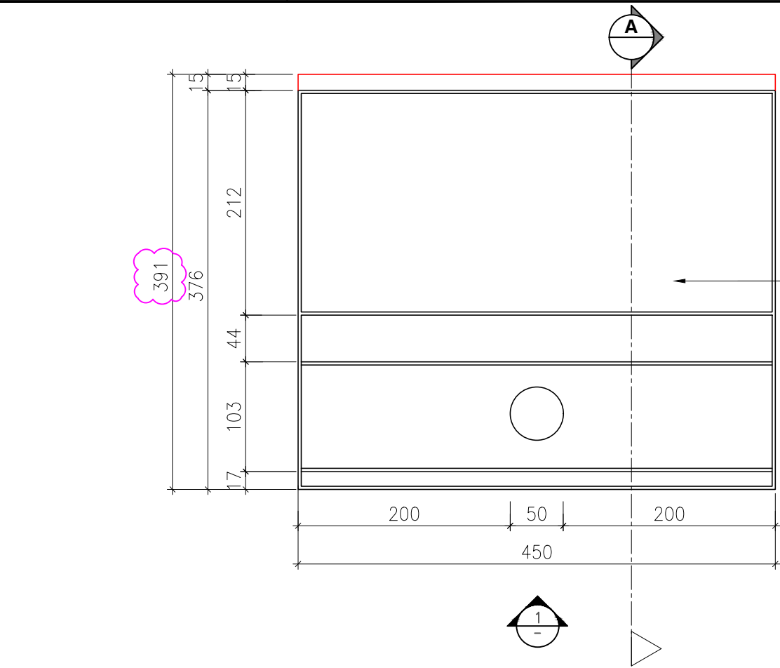
1 PLAN SCALE 1:5
