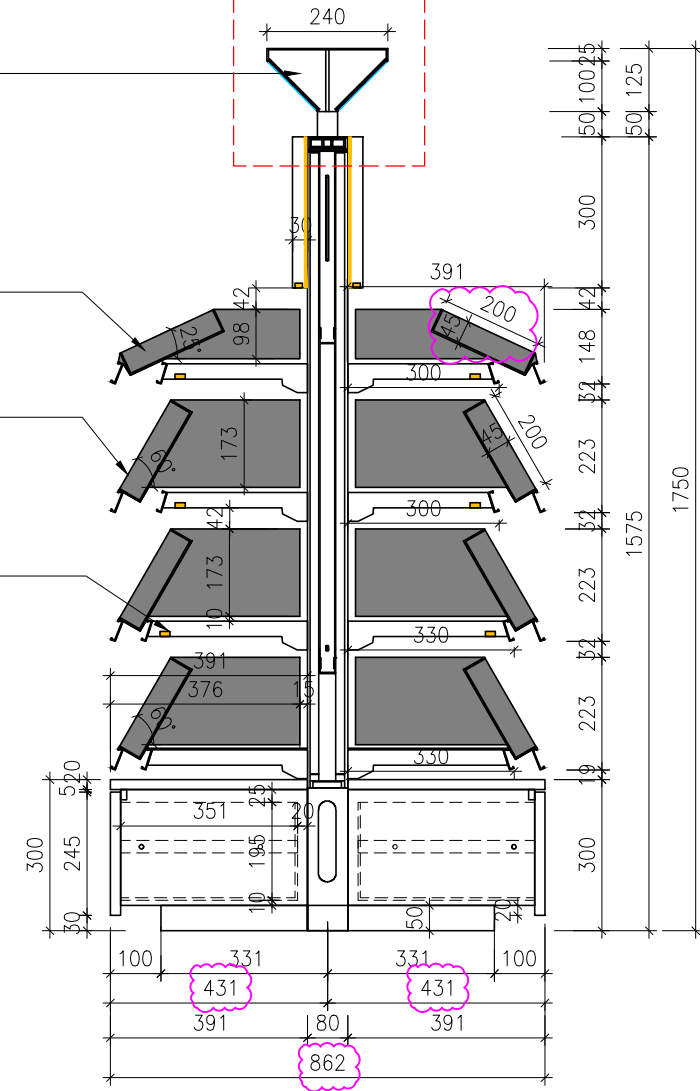
3 SECTION A SCALE 1:15
