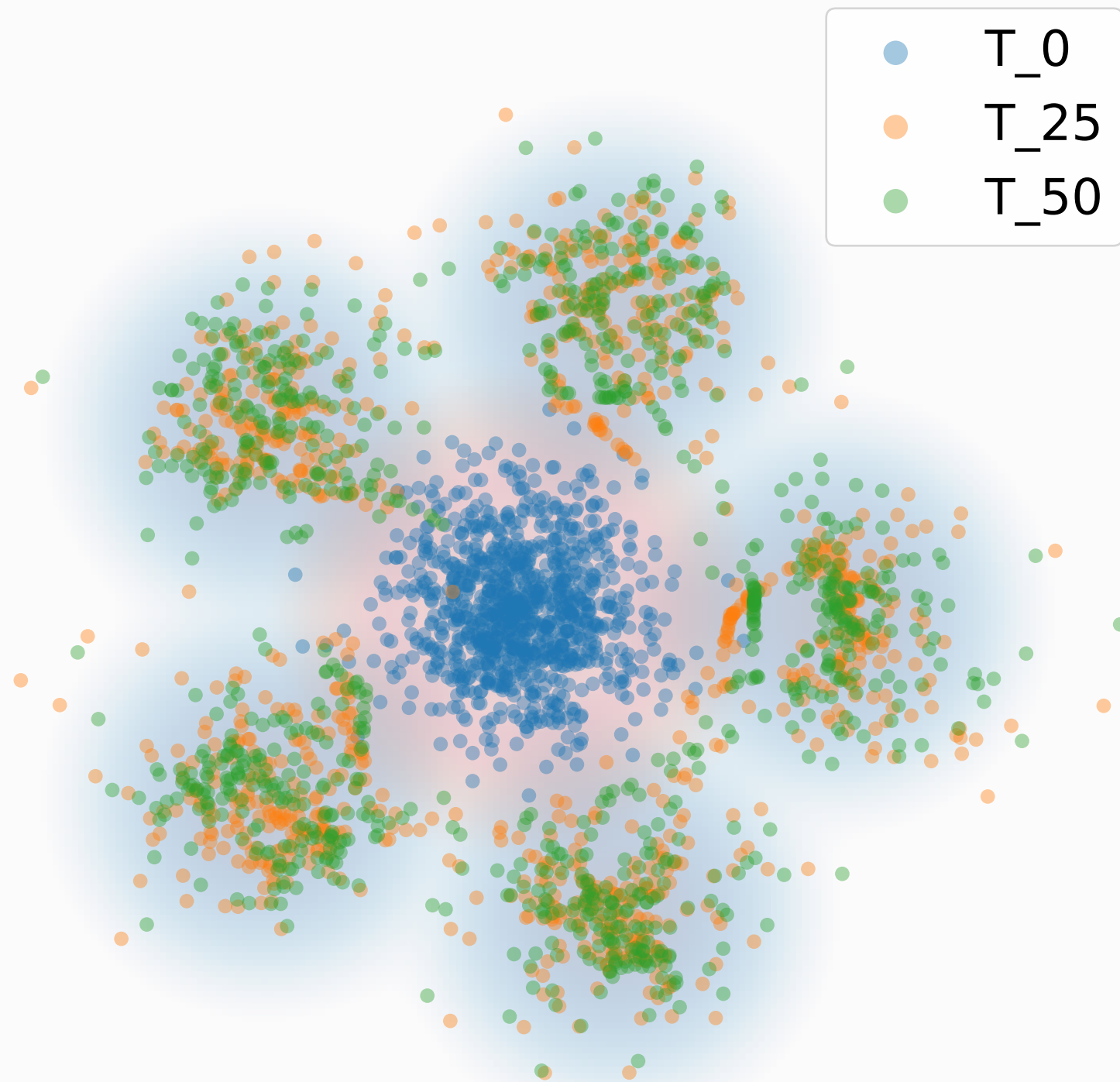
Samples from Learned Marginal ODE
