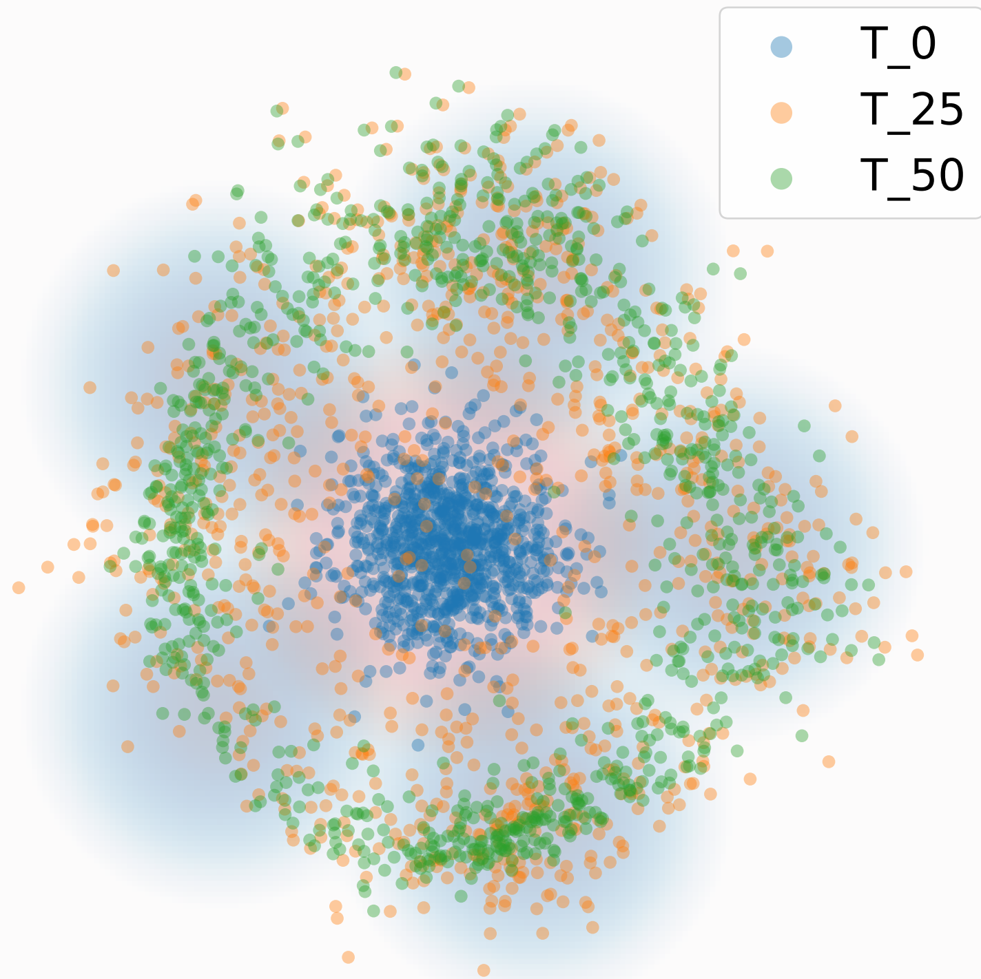
Samples from Learned Marginal ODE
