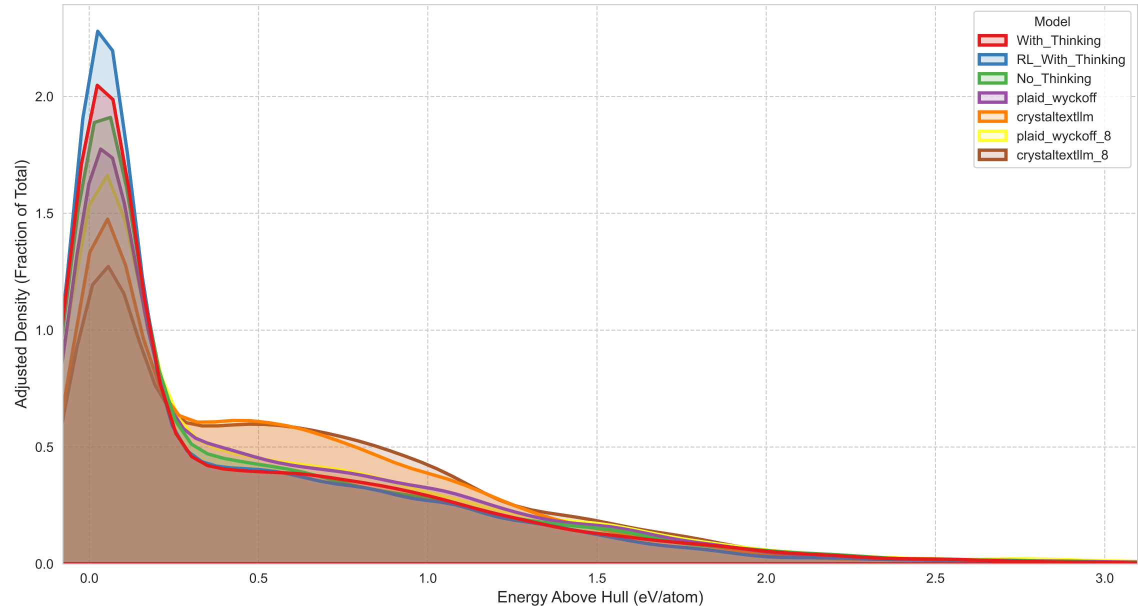
Energy Above Hull Distribution (Normalized by Total Samples)
