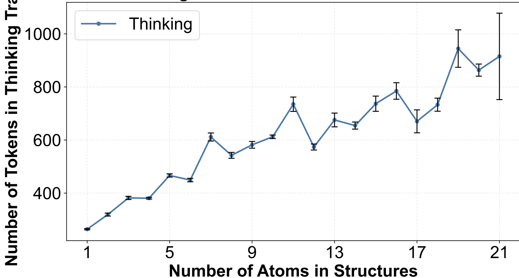
Thinking Trace Token Count vs Atom Count
