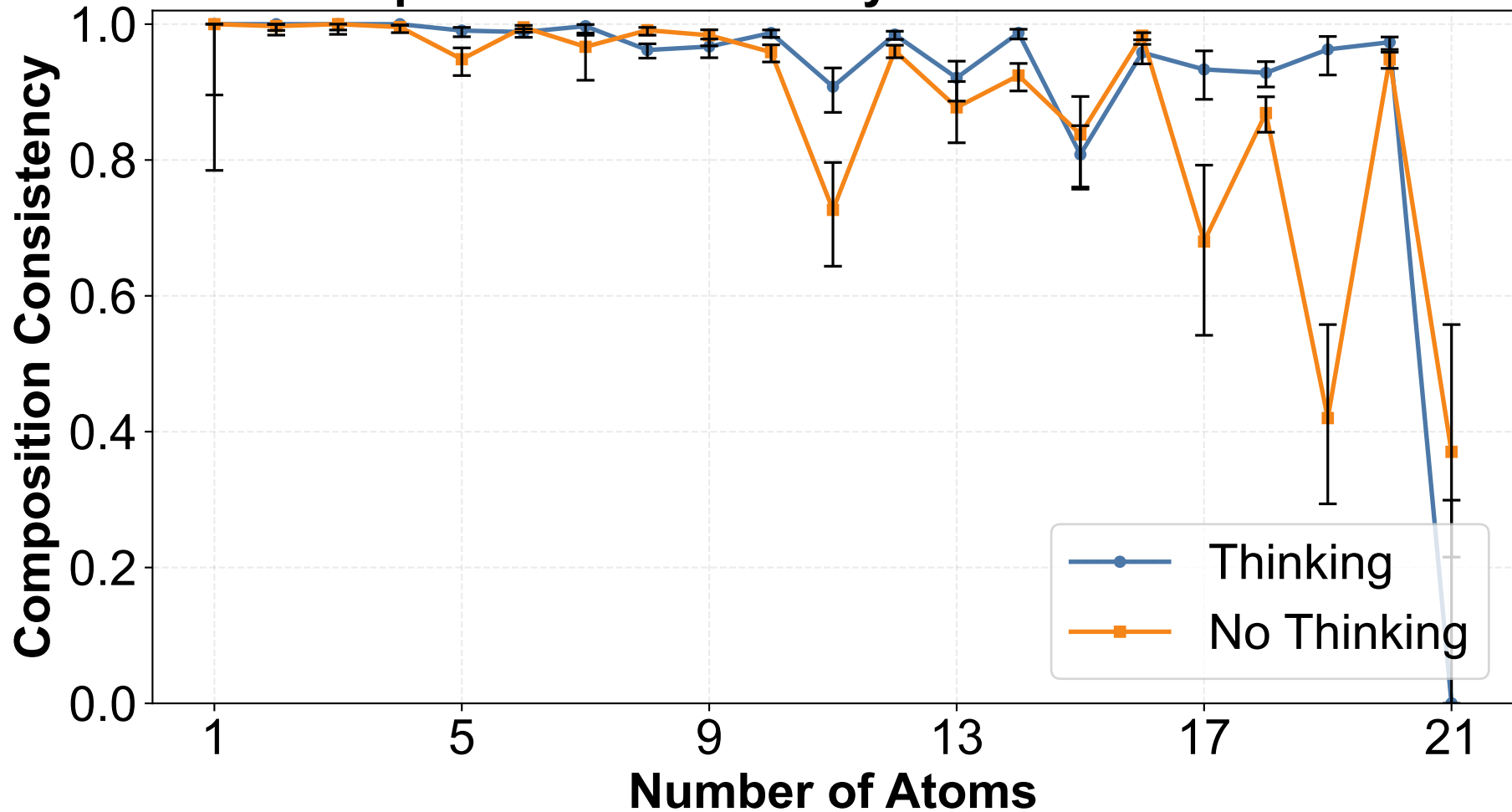
Composition Consistency vs Number of Atoms
