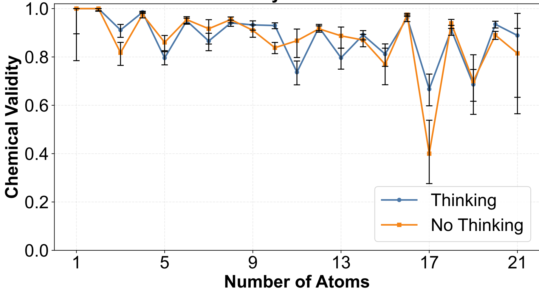
Chemical Validity vs Number of Atoms
