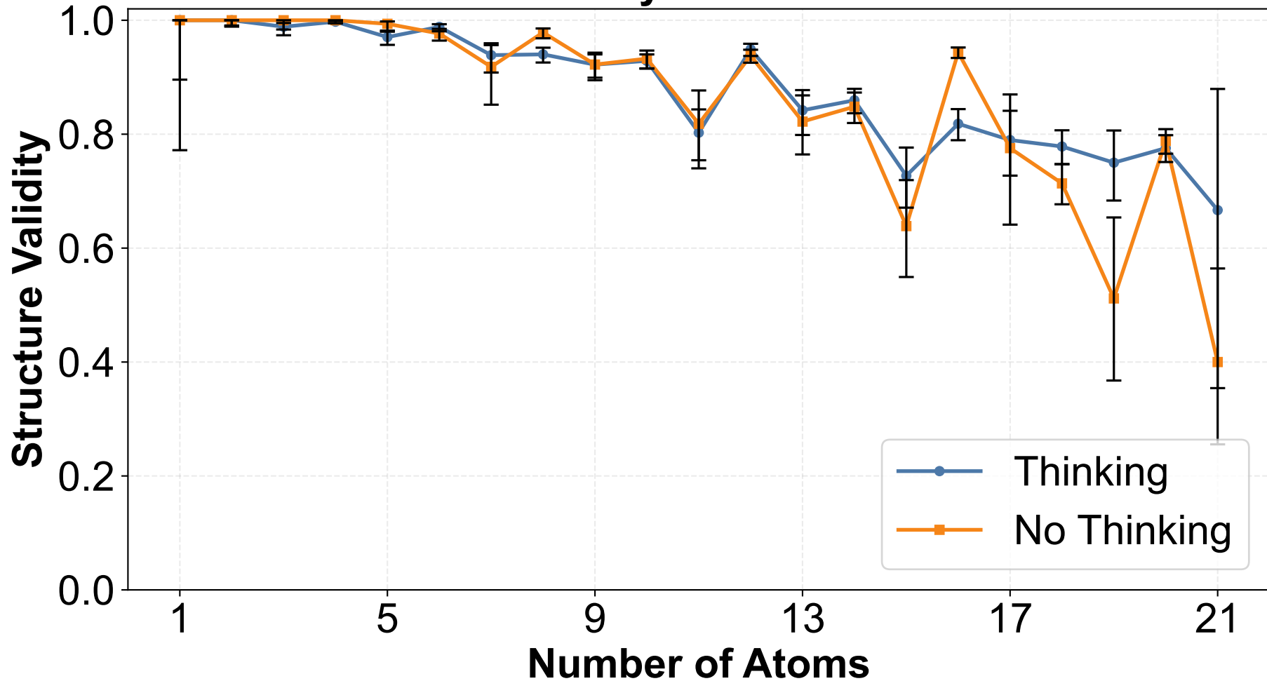
Structure Validity vs Number of Atoms
