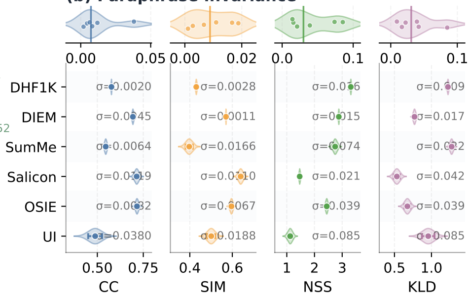
(b) Paraphrase invariance
