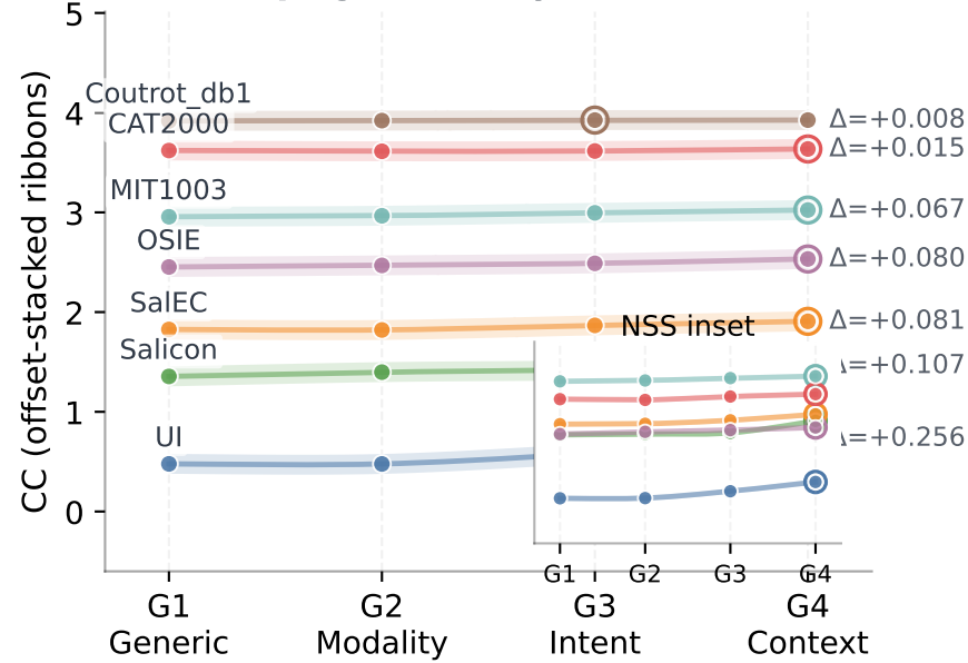
(c) Prompt granularity
