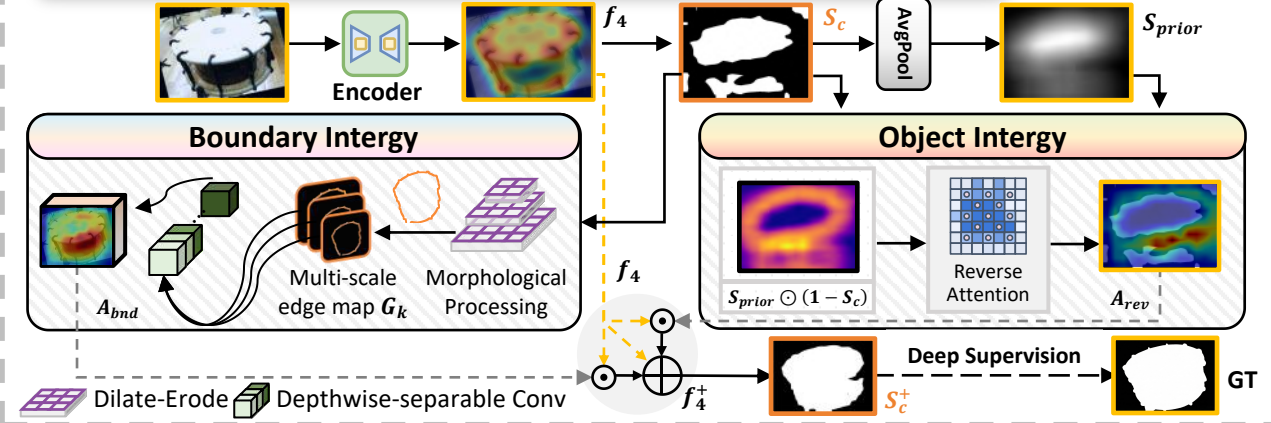
(c) Synergistic Integrity Refinement Module (SIR)
