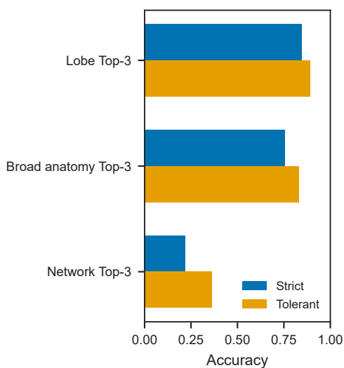
B Paired MRI baseline
