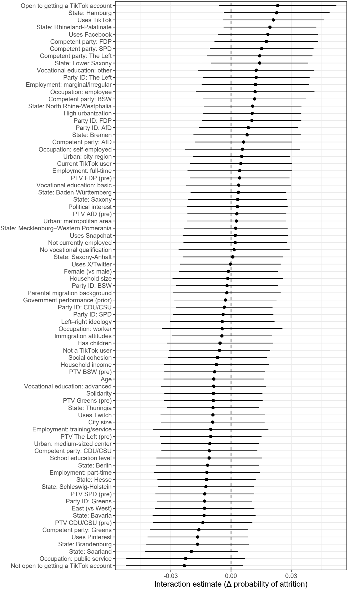
Treatment × covariate interactions on attrition (LPM)
