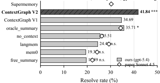
SWE-ContextBench Lite, n=98 paired, gpt-5.4 base agent
