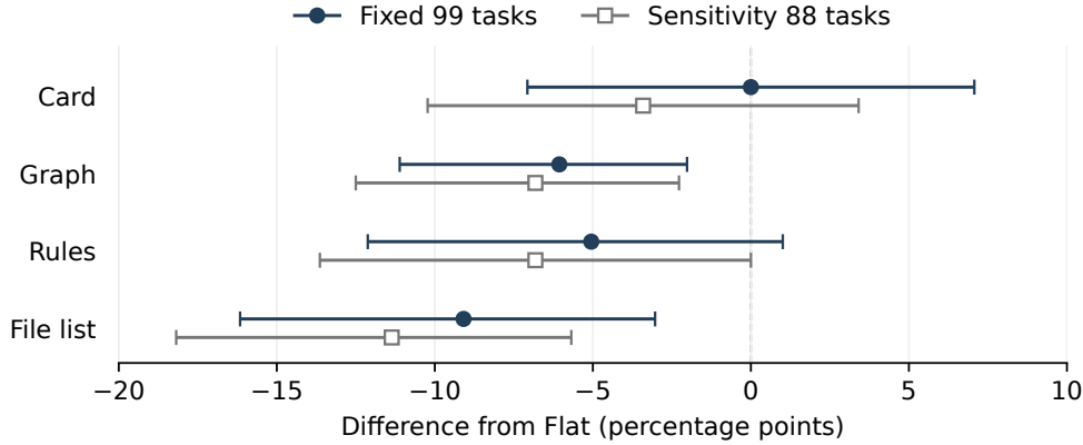
Figure 1: Archived Related-Lite first-prediction repair differences relative to Flat, on the full 99 tasks and the pre-existing 88-task source-overlap sensitivity set. Bars are unadjusted 95% paired bootstrap intervals. These retrospective comparisons include operational failures and retain the historical receipt limitation; they do not isolate causal memory effects.
