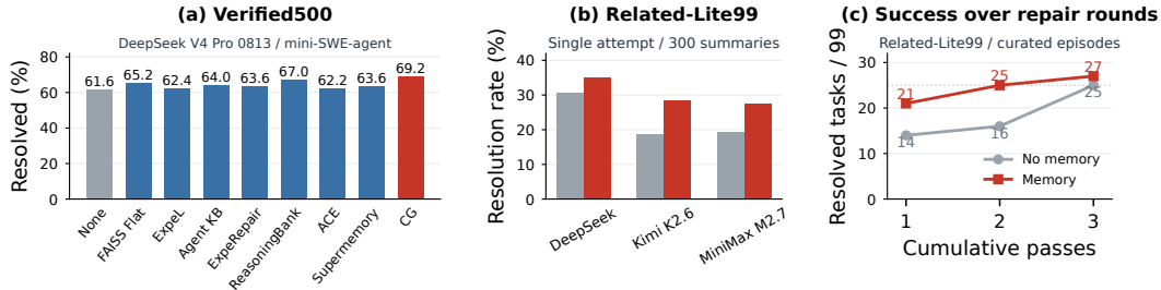
Figure 1: ContextGraph improves repair success across the evaluated settings. (a) SWE-bench Verified500 with DeepSeek V4 Pro 0813 and mini-SWE-agent; (b) Related-Lite99 with three language models; (c) cumulative resolutions on Related-Lite99 with DeepSeek V4 Pro. Grey denotes no memory and red ContextGraph.
