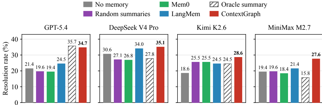
Figure 5: Related-Lite99 resolution (resolved/completed, %), one attempt per task and 300 summaries per model. ContextGraph is red; the hatched oracle receives a known related summary.
