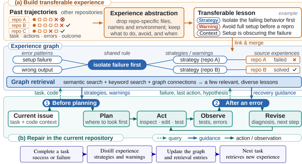
Figure 3: ContextGraph’s experience-memory architecture. Past trajectories supply strategies and warnings linked to source context. The agent retrieves guidance before planning and after errors. After every task, successful and failed trajectories update the graph; the added experience is immediately available to subsequent tasks. Graph links illustrate the organization.
