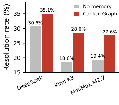
(b) Across models
