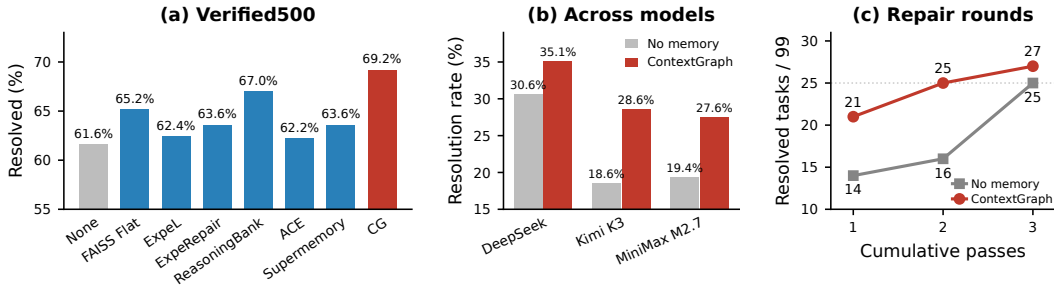
Figure 1: ContextGraph improves repair success across the evaluated settings. (a) SWE-bench Verified500 with DeepSeek V4 Pro 0813 and mini-SWE-agent; (b) Related-Lite99 with three language models, one attempt per task and 300 summaries; (c) cumulative resolutions over repair rounds on Related-Lite99 with DeepSeek V4 Pro and curated episodic memory. Grey denotes no memory and red ContextGraph.
