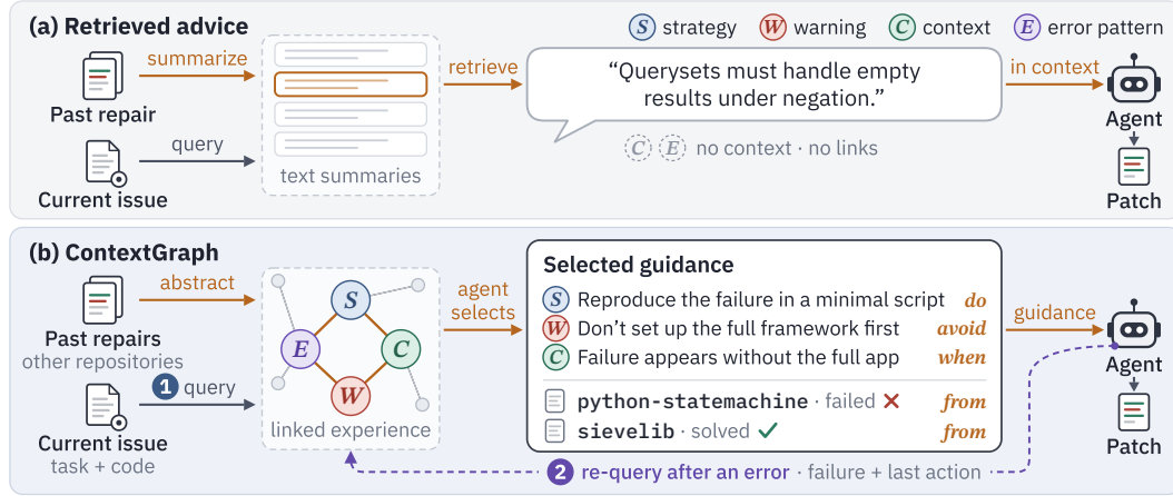
Figure 2: Retrieved advice versus ContextGraph on the Django example above (illustration). (a) Flat summaries return one requirement sentence without context or source. (b) The agent selects a strategy, a warning, and their applicability condition, linked to the failed python-statemachine and the successful sievelib attempts, before planning and again after an error.
