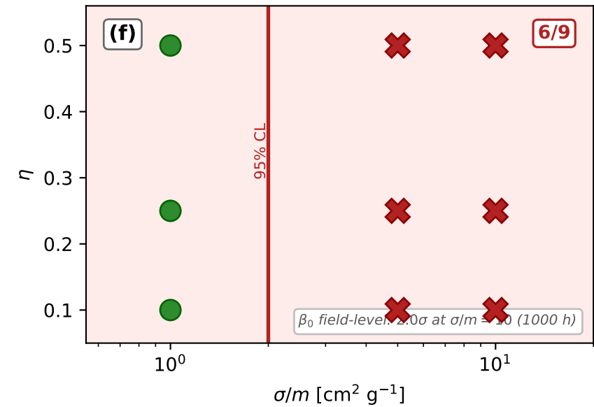
21 cm power spectrum P_{21}(k) SKA1-Low, 1000 hr (optimistic)
