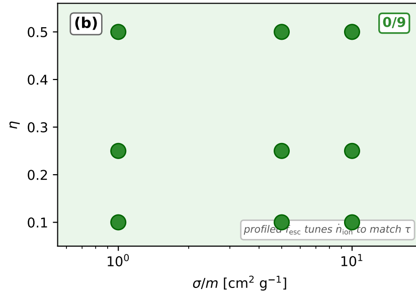
Thomson optical depth Planck, \tau = 0.054 \pm 0.007
