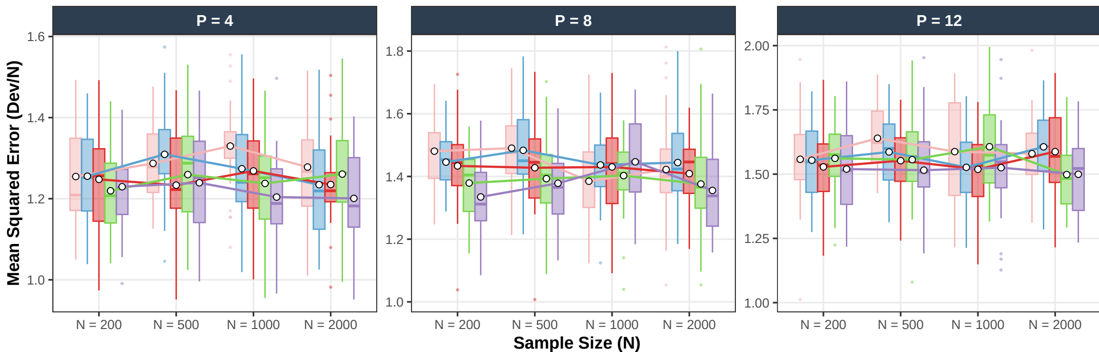
B. Impact of Sample Size on Model Fit
