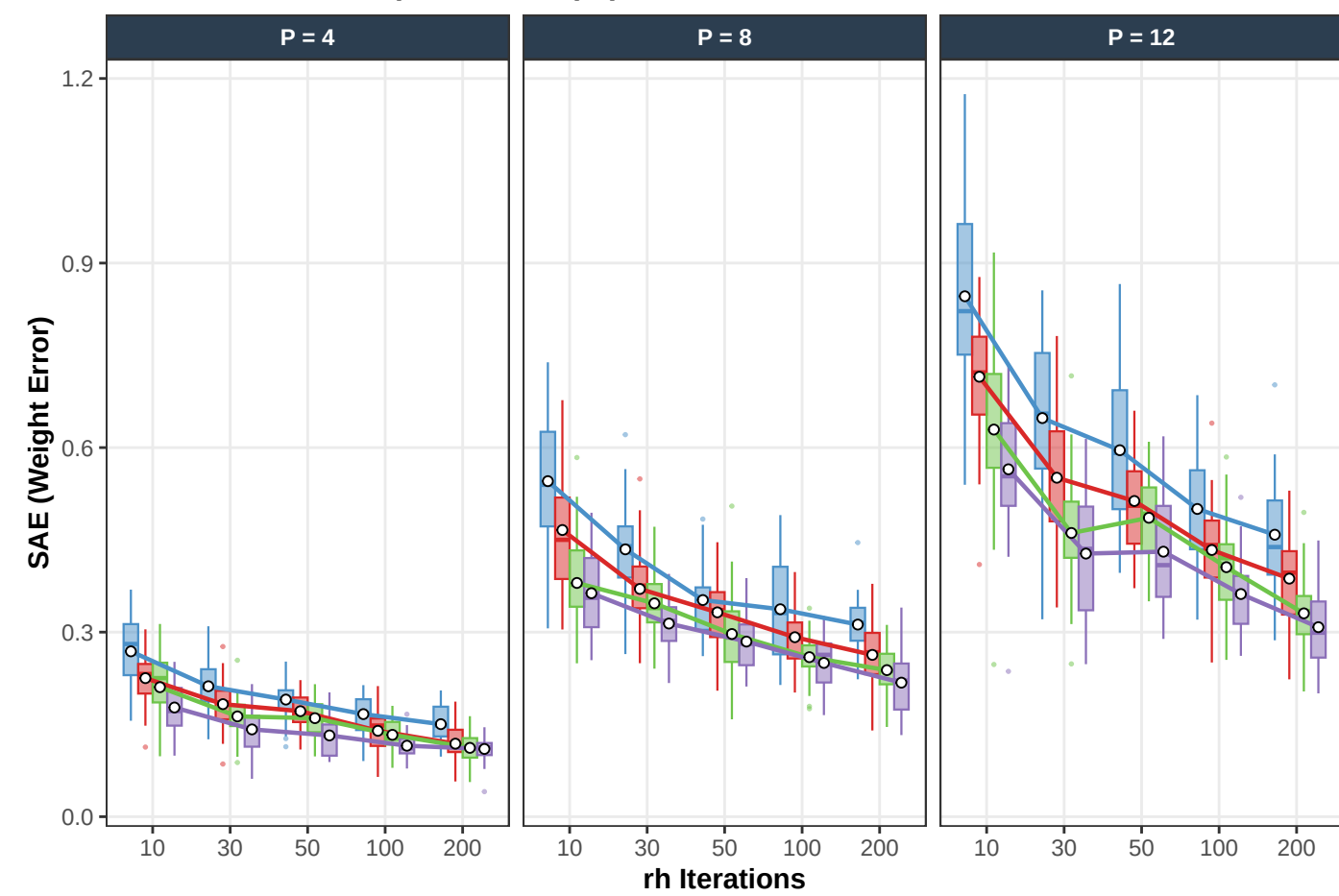
D. Fit Error vs. Bootstrap Iterations (rh)
