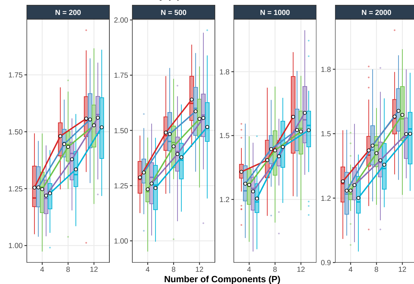
F. Fit Error vs. Dimensionality (P)
