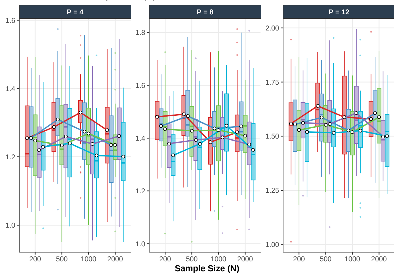
E. Fit Error vs. Sample Size (N)
