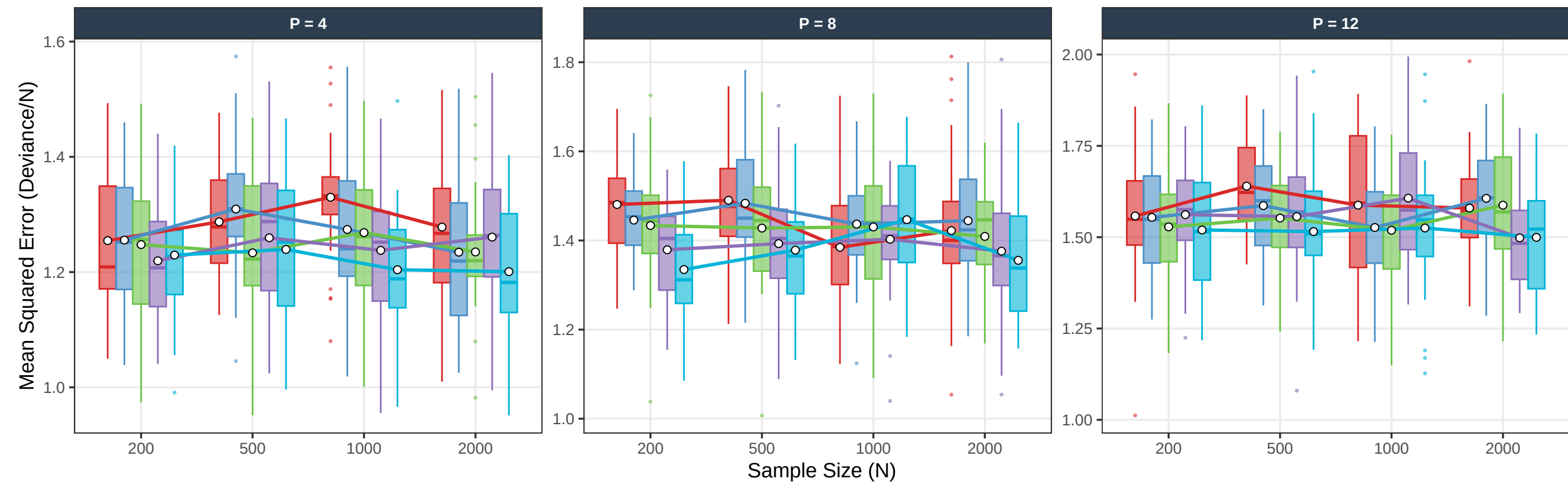
D. Fit Error: Impact of Sample Size (N)
