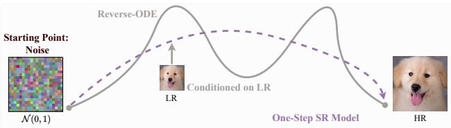
(b) Our Noise-Started One-Step Diffusion for Real-ISR. Starting from random Gaussian noise, our method performs one-step HR generation with LR conditioning, achieving efficient inference and strong perceptual quality.
