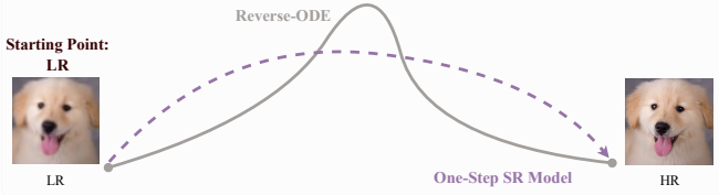
(a) Vanilla One-Step Diffusion for Real-ISR. The HR image is directly restored from the LR input in a single step, improving efficiency but sacrificing stochasticity and perceptual quality.
