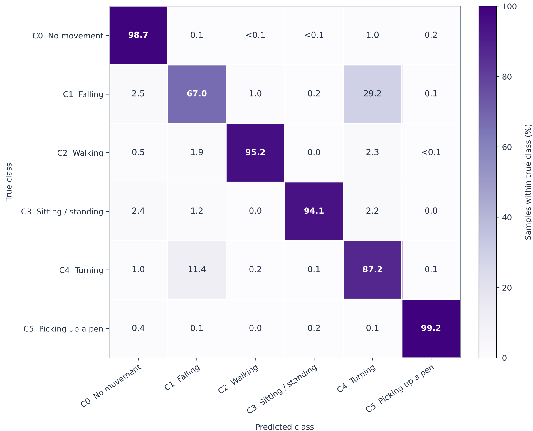
H11 residual TPP + SupCon: all-class confusion matrix E1-E3 × seeds 42/52/62 · row-normalized
