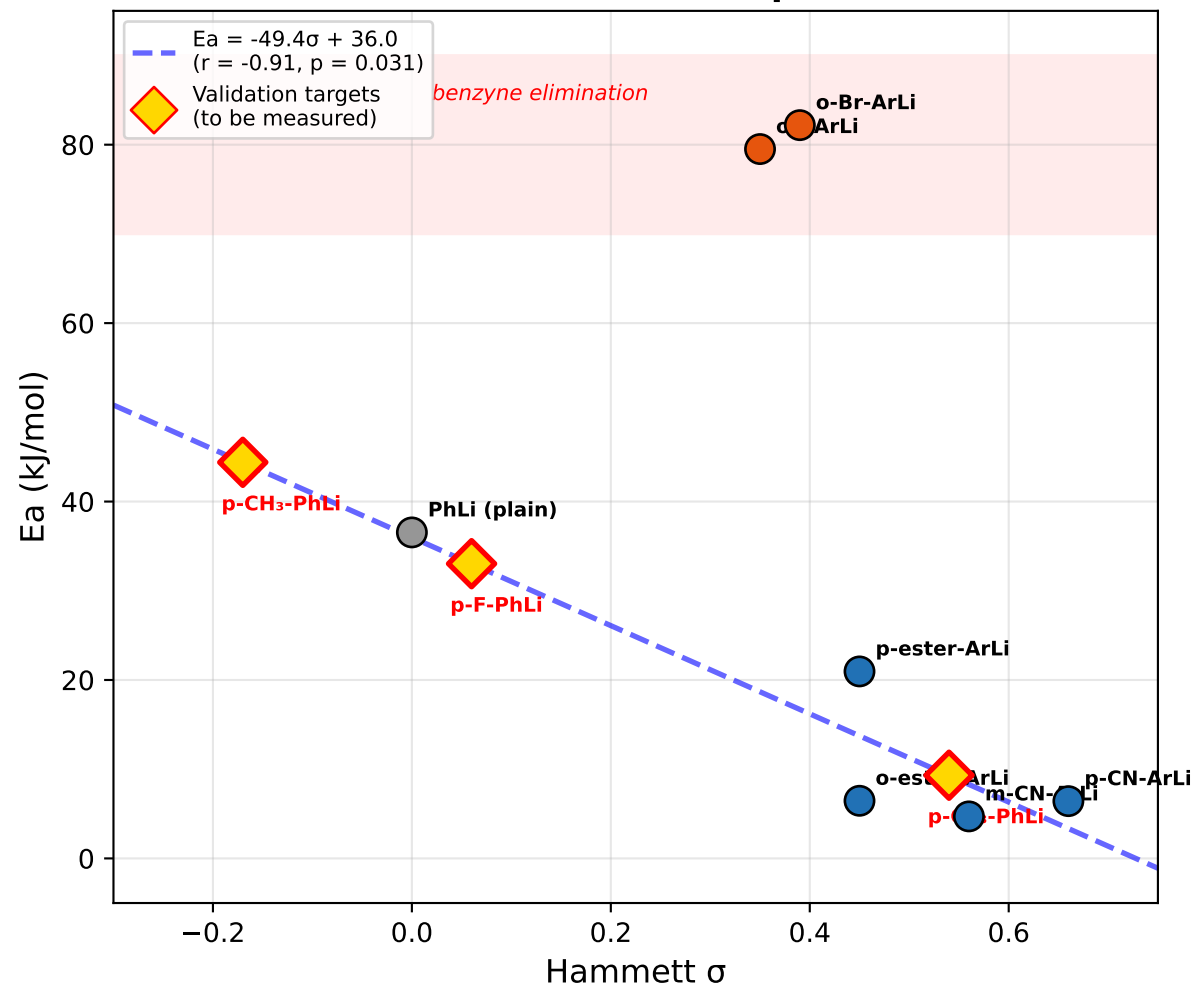
(a) Hammett \sigma vs Decomposition E_a
