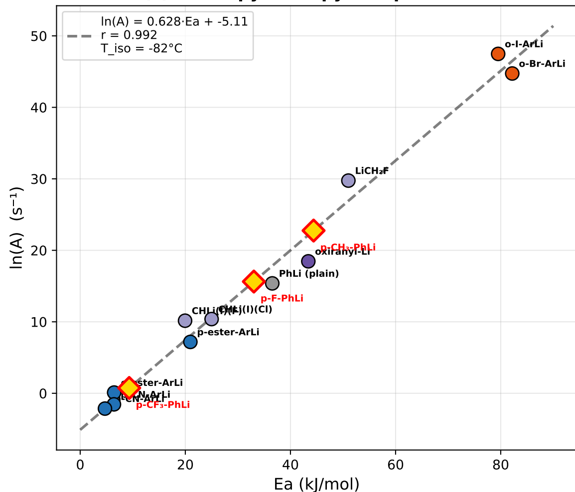
(c) Enthalpy-Entropy Compensation
