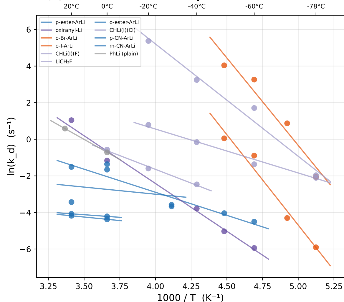
(b) Arrhenius Plot: Decomposition Rate Constants
