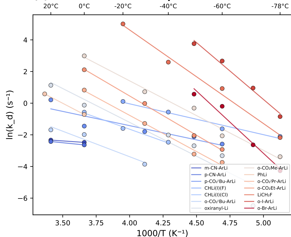
(a) Arrhenius Plot: Decomposition Rate Constants
