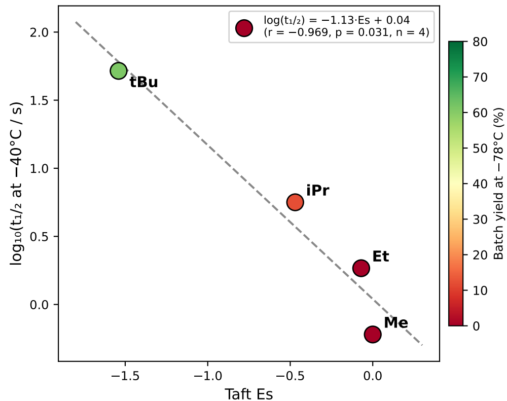
(c) Taft Steric Effect on Ortho-Ester ArLi
