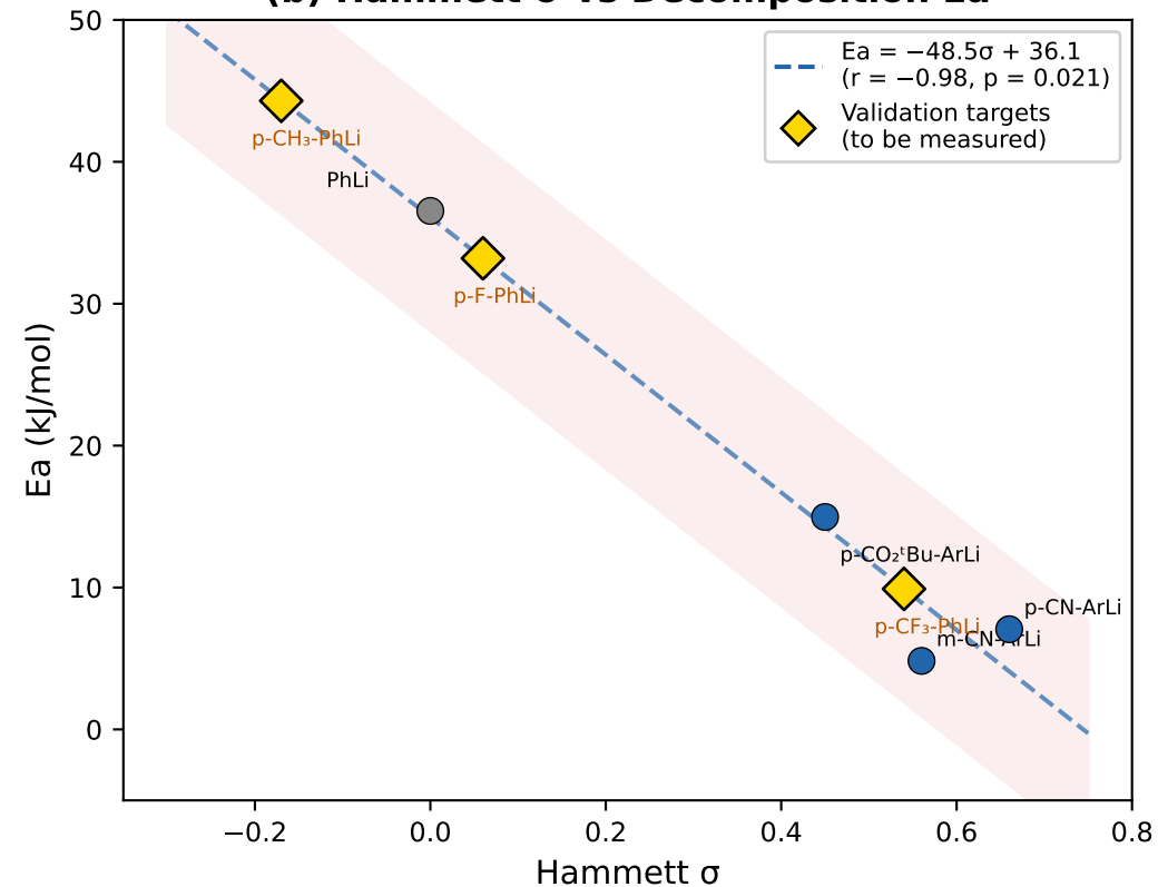
(b) Hammett \sigma vs Decomposition Ea
