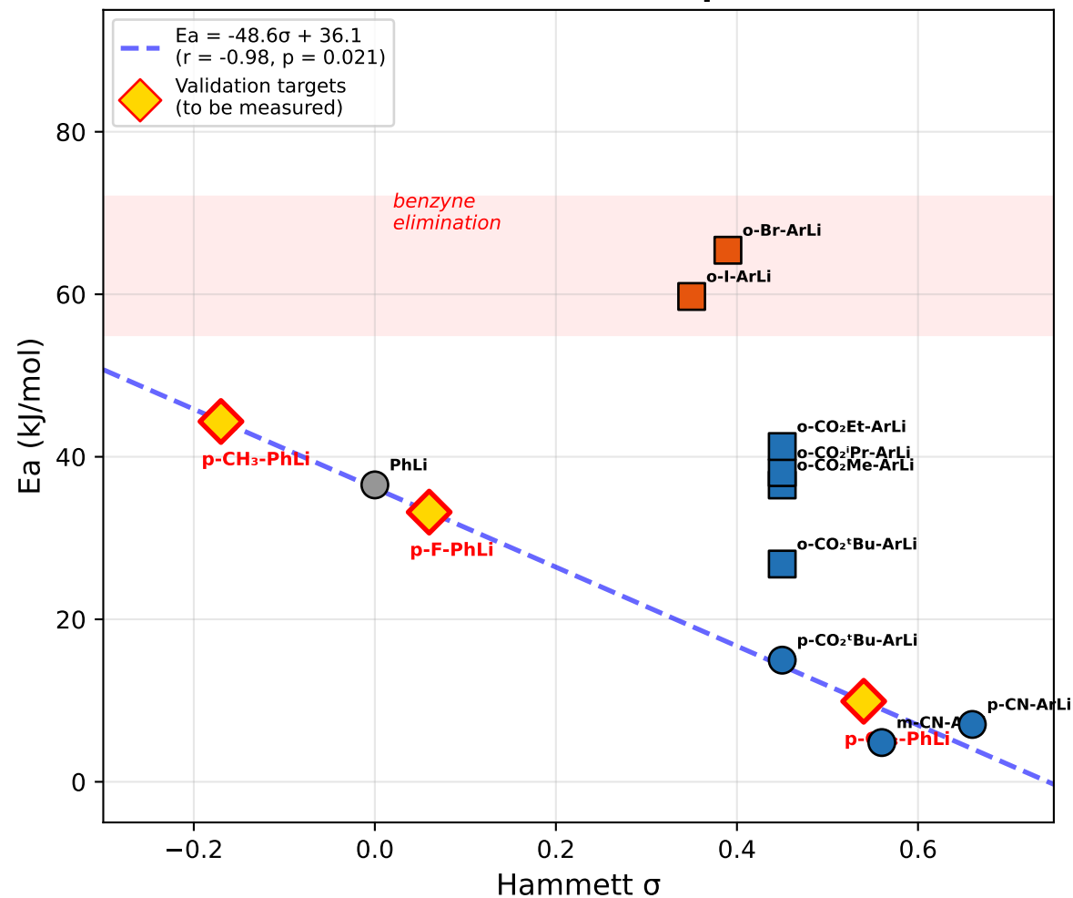
(a) Hammett \sigma vs Decomposition Ea
