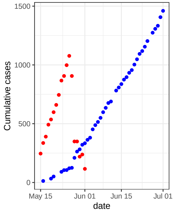
Cumulative cases
