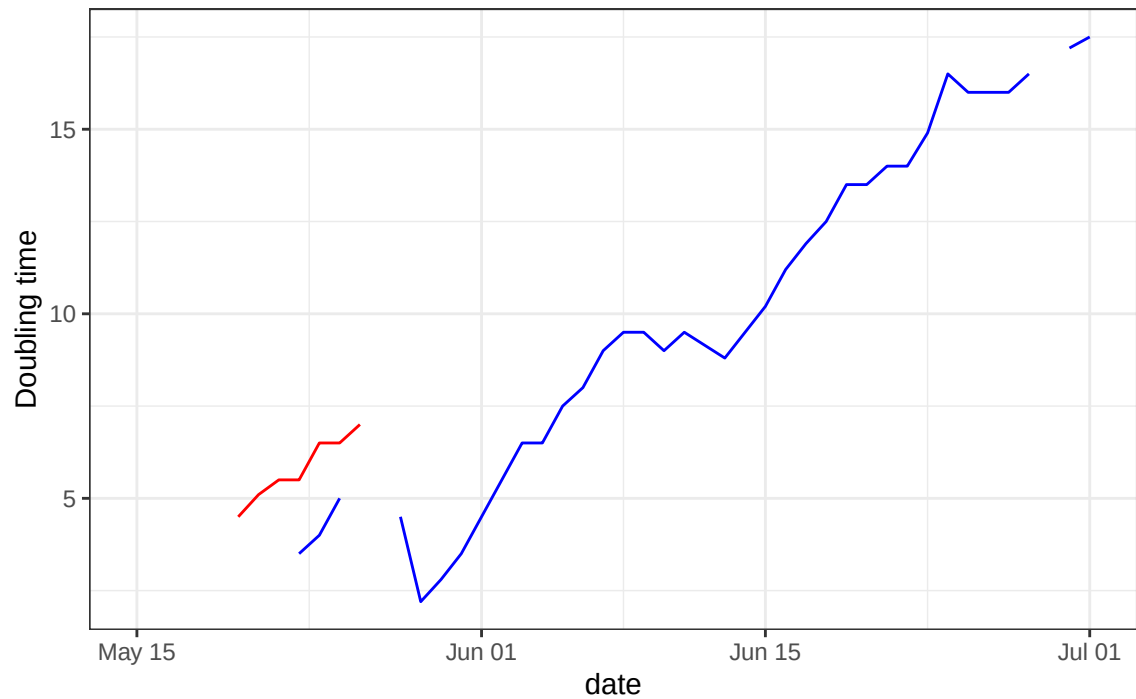
Doubling time
