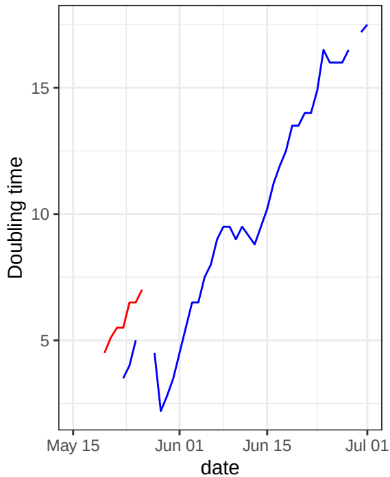
Doubling time
