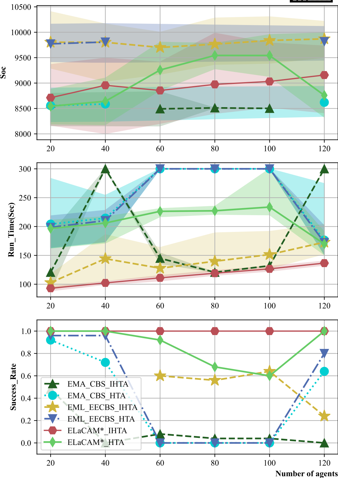
room-32-32-4 32x32 ( |V|=682 ) |T|=200 Runtime limit=300
