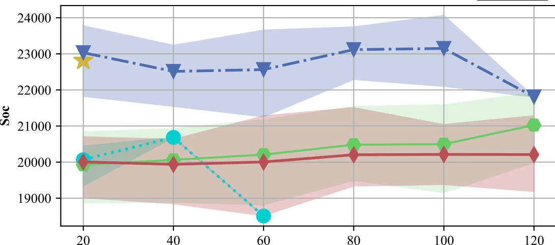
room-64-64-8 64x64 ( |V|=3232 ) |T|=200 Deadline=700
