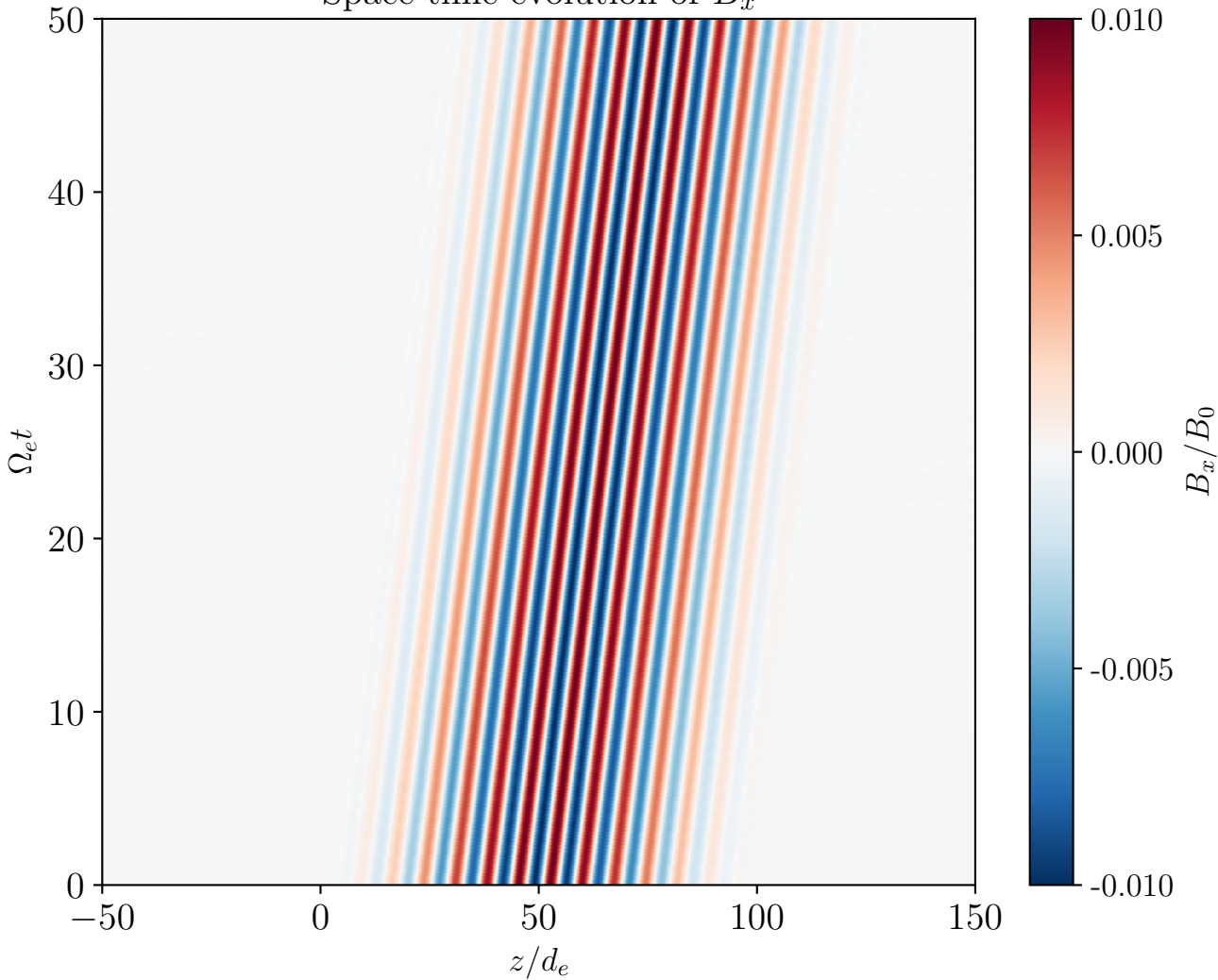
Space-time evolution of B_x
