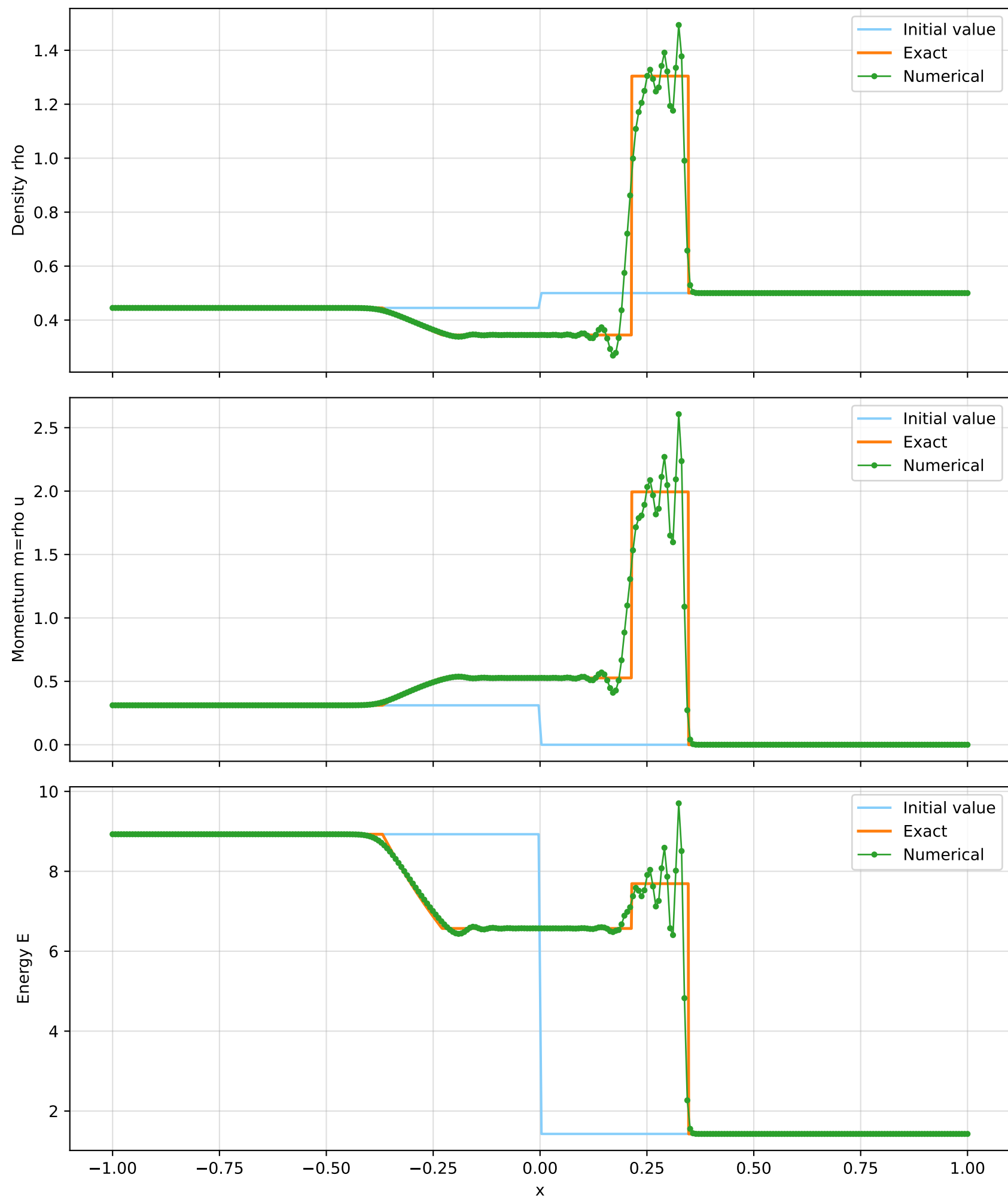
Fig 1: Lax-Wendroff (300 grids, CFL=0.22)
