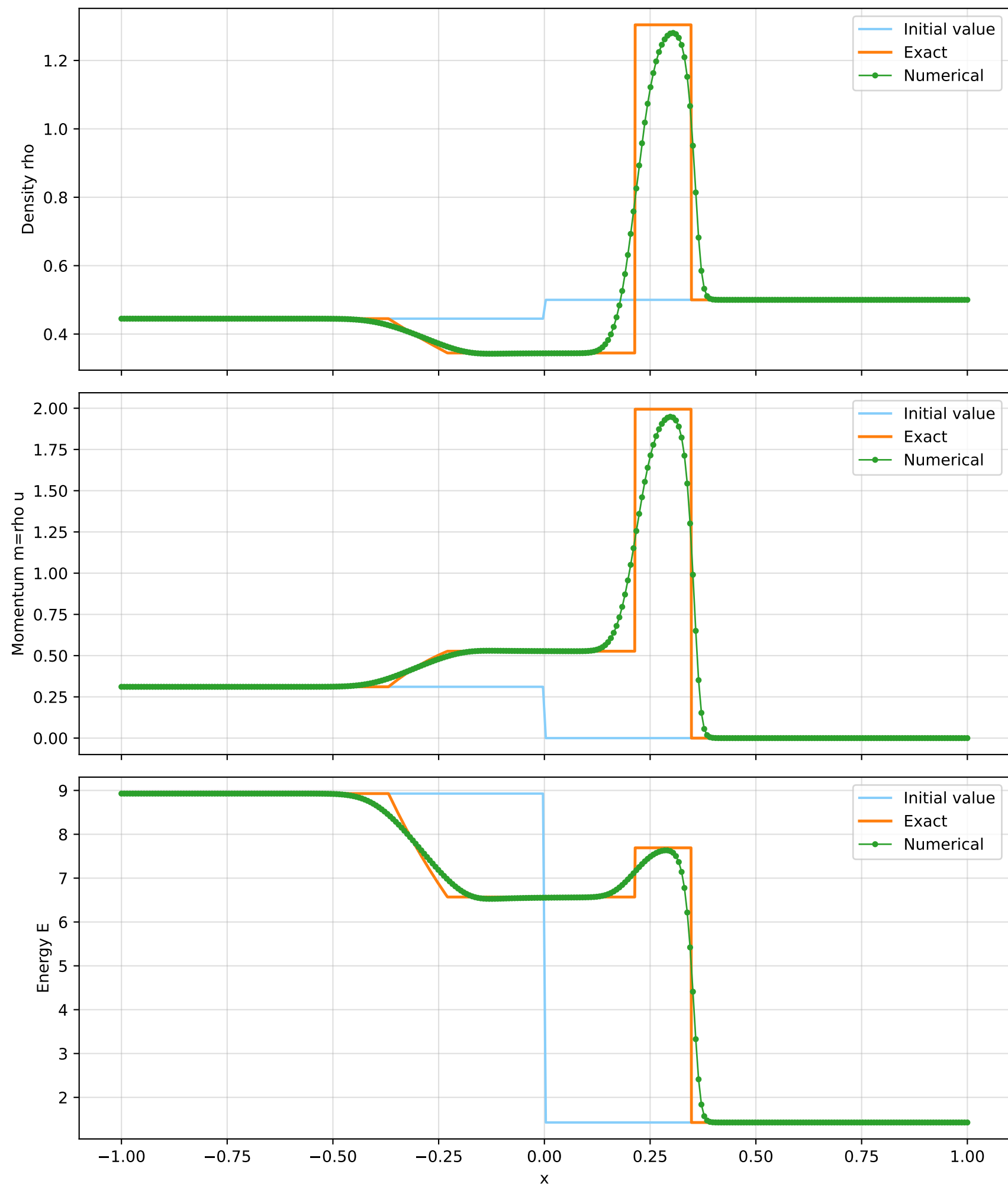
Fig 2: TVD (300 grids, CFL=0.1)
