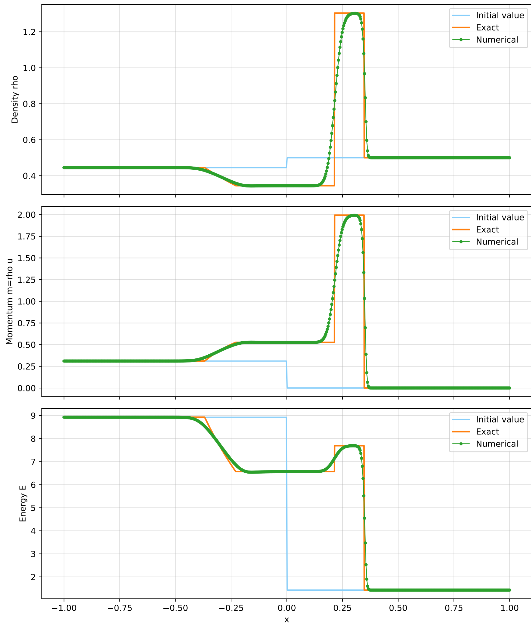
Fig 3: TVD (600 grids, CFL=0.1)
