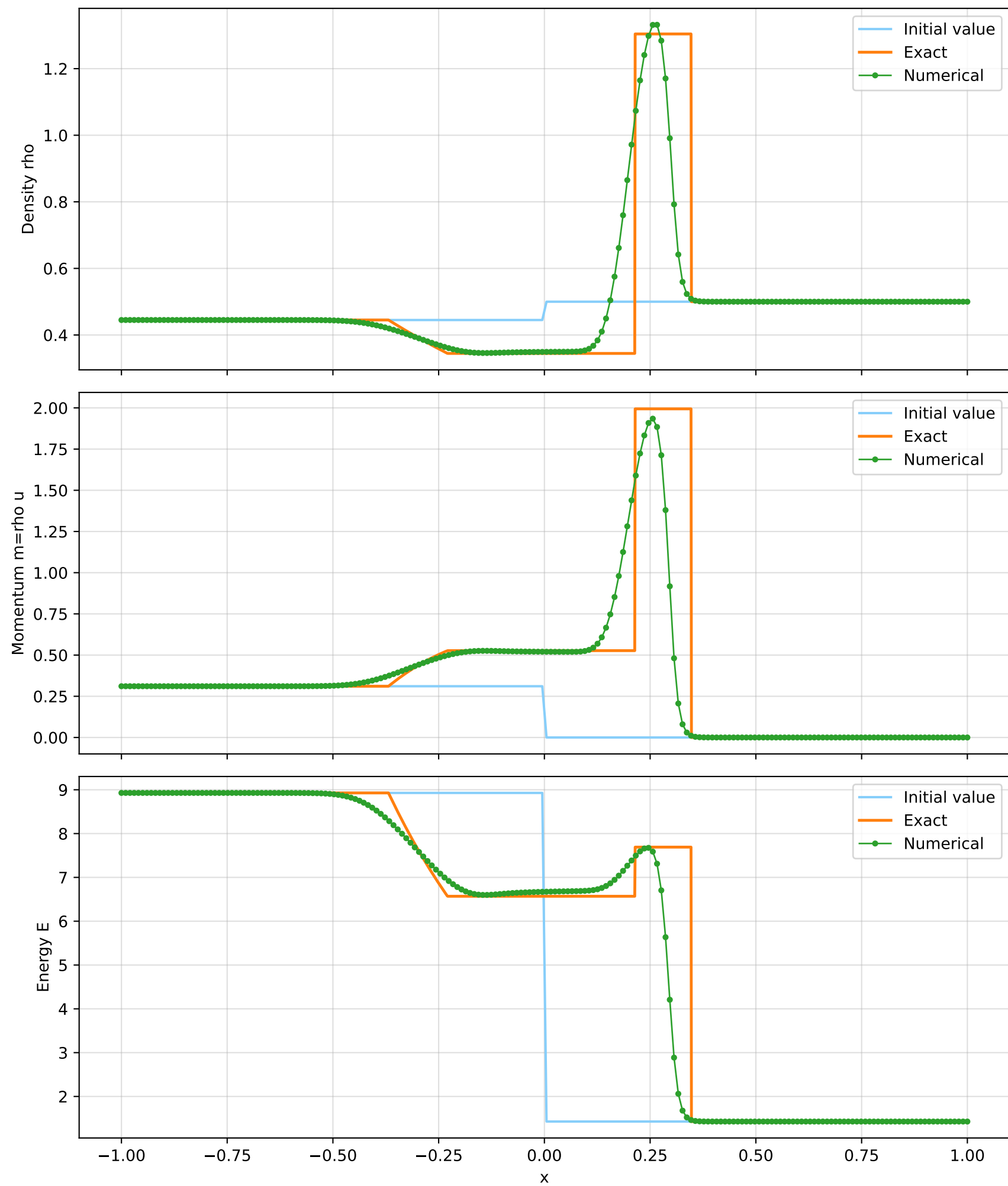
Fig 4: Upwind (200 grids, CFL=0.01)
