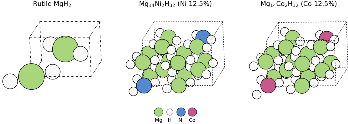
Figure 1: Relaxed product structures: pristine rutile \text{MgH}_2 (left), \text{Mg}_{14}\text{Ni}_2\text{H}_{32} (centre), and \text{Mg}_{14}\text{Co}_2\text{H}_{32} (right), the latter two at 12.5 at.% substitution. In the doped cells the two transition-metal atoms occupy diagonally opposite Mg sites in the 2 \times 2 \times 2 rutile supercell, maximising their separation to minimise dopant–dopant interaction.
