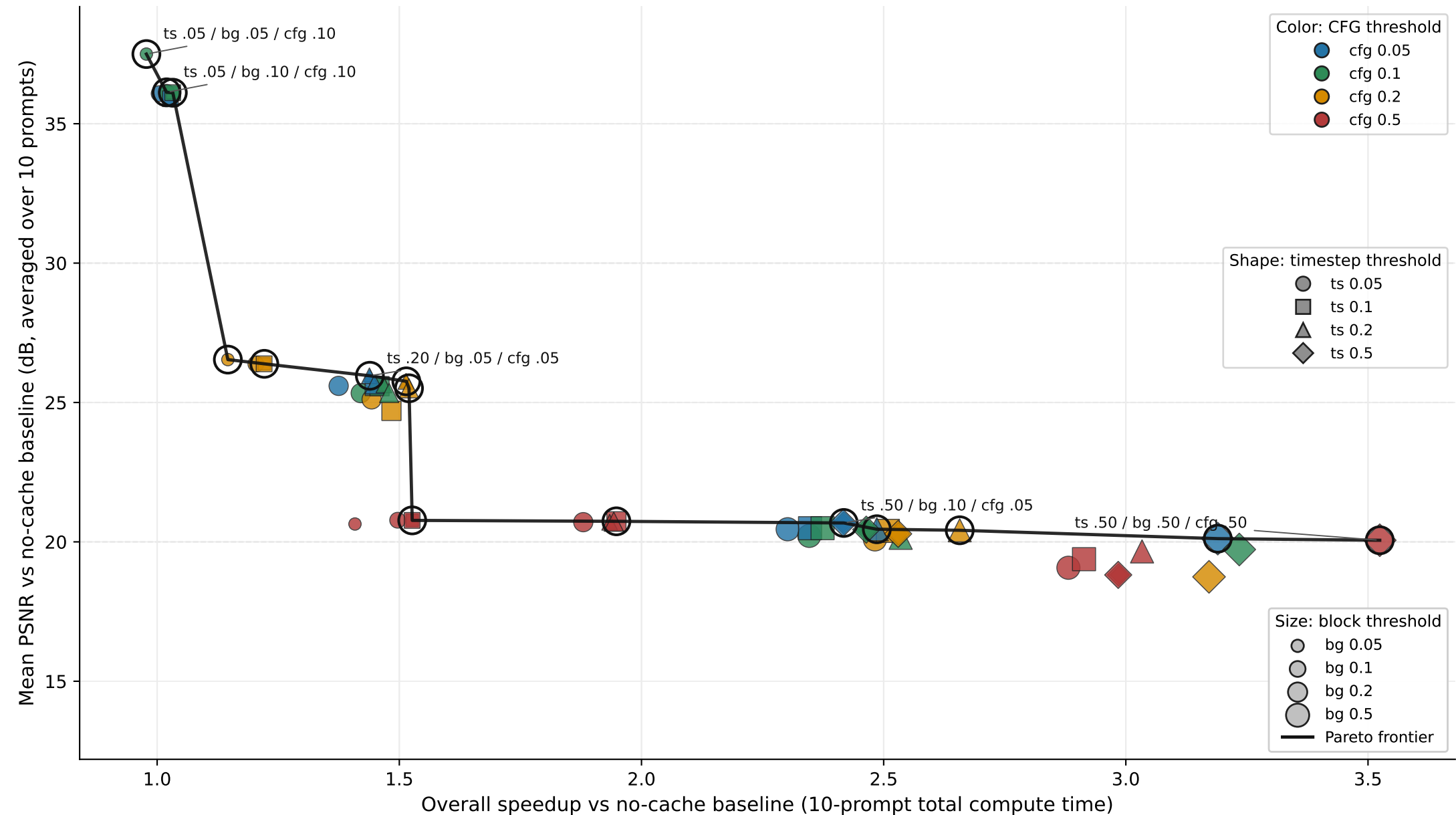
VBench10 Three-Cache Threshold Combinations: PSNR-Speedup Pareto Scatter
