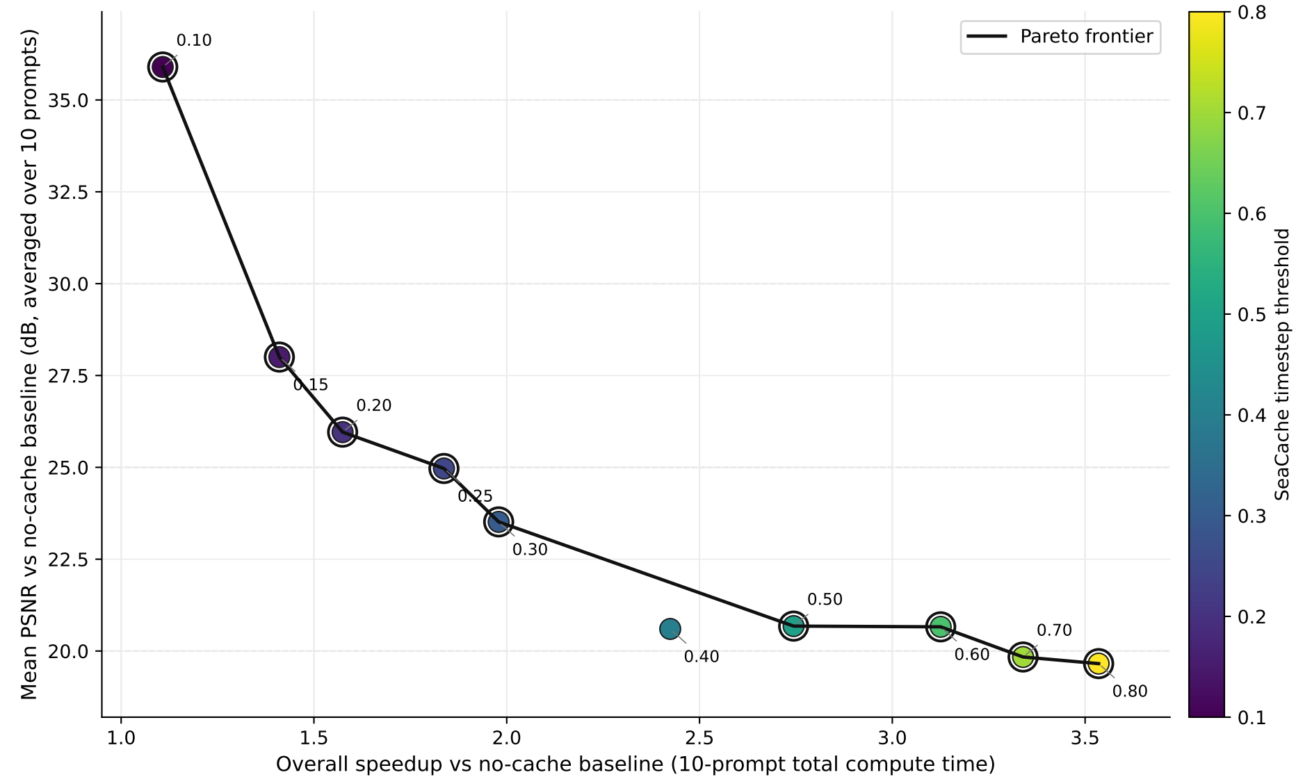
VBench10 Timestep-Only SeaCache: PSNR-Speedup Pareto Scatter
