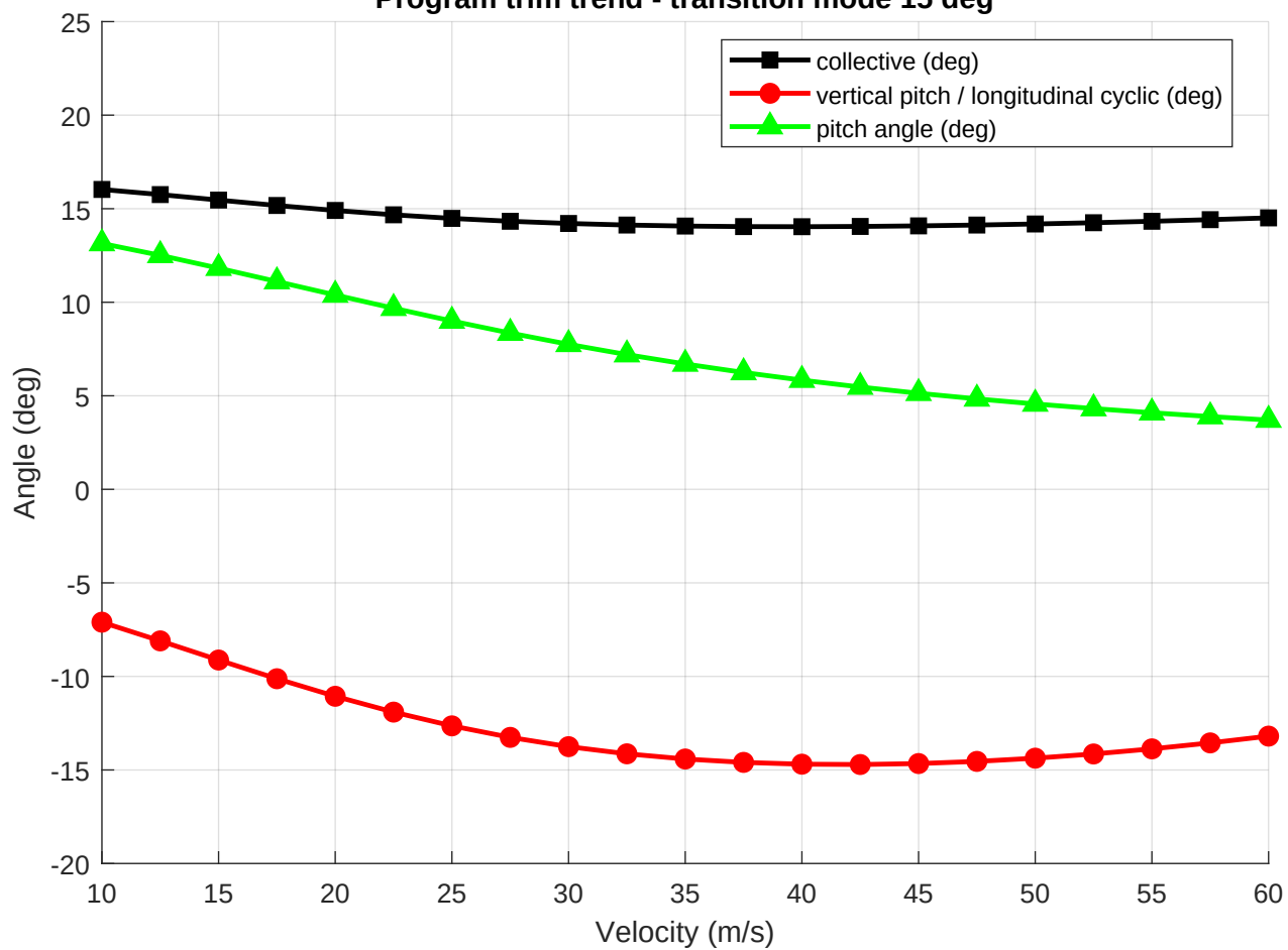
Program trim trend - transition mode 15 deg
