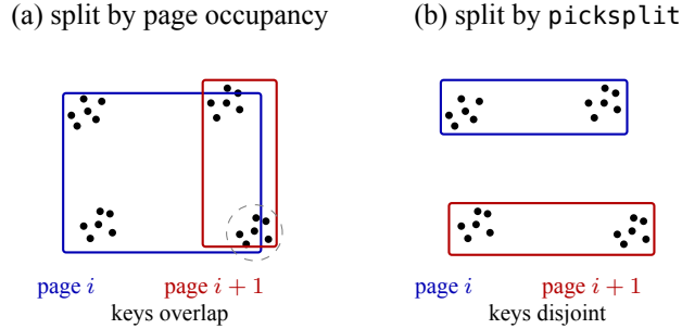
Figure 1: The same entries under the same order; only the choice of page boundaries differs. Filling each page to capacity (a) puts the boundary in the middle of a dense region, so the bounding keys of two neighbouring pages cover almost the same area and a query matching either enters both subtrees. Delegating the choice to the operator class (b) lets boundaries follow the data and the keys come out disjoint. Rectangles are the keys stored in the parent.
