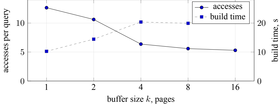
Figure 3: Dependence on the buffer size, N = 10^7 uniform points. k = 1 reproduces occupancy-based packing. The value shipped in PostgreSQL, k = 4 , is conservative: k = 8 improves query cost by 12 % at no cost in build time.
