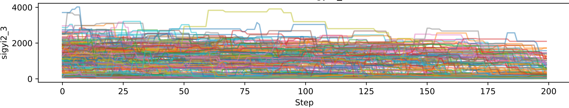
Chain for sigyi2_3
