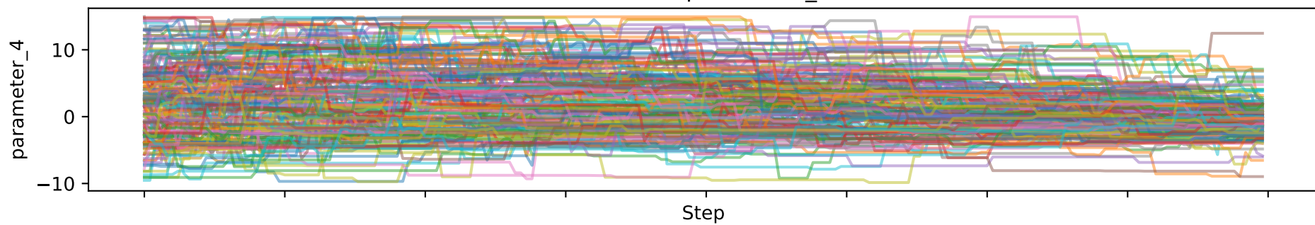
Chain for sigyi2_1
