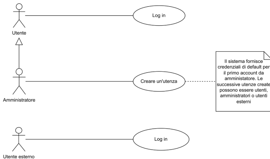
Figura 1.1: Login use case diagram
