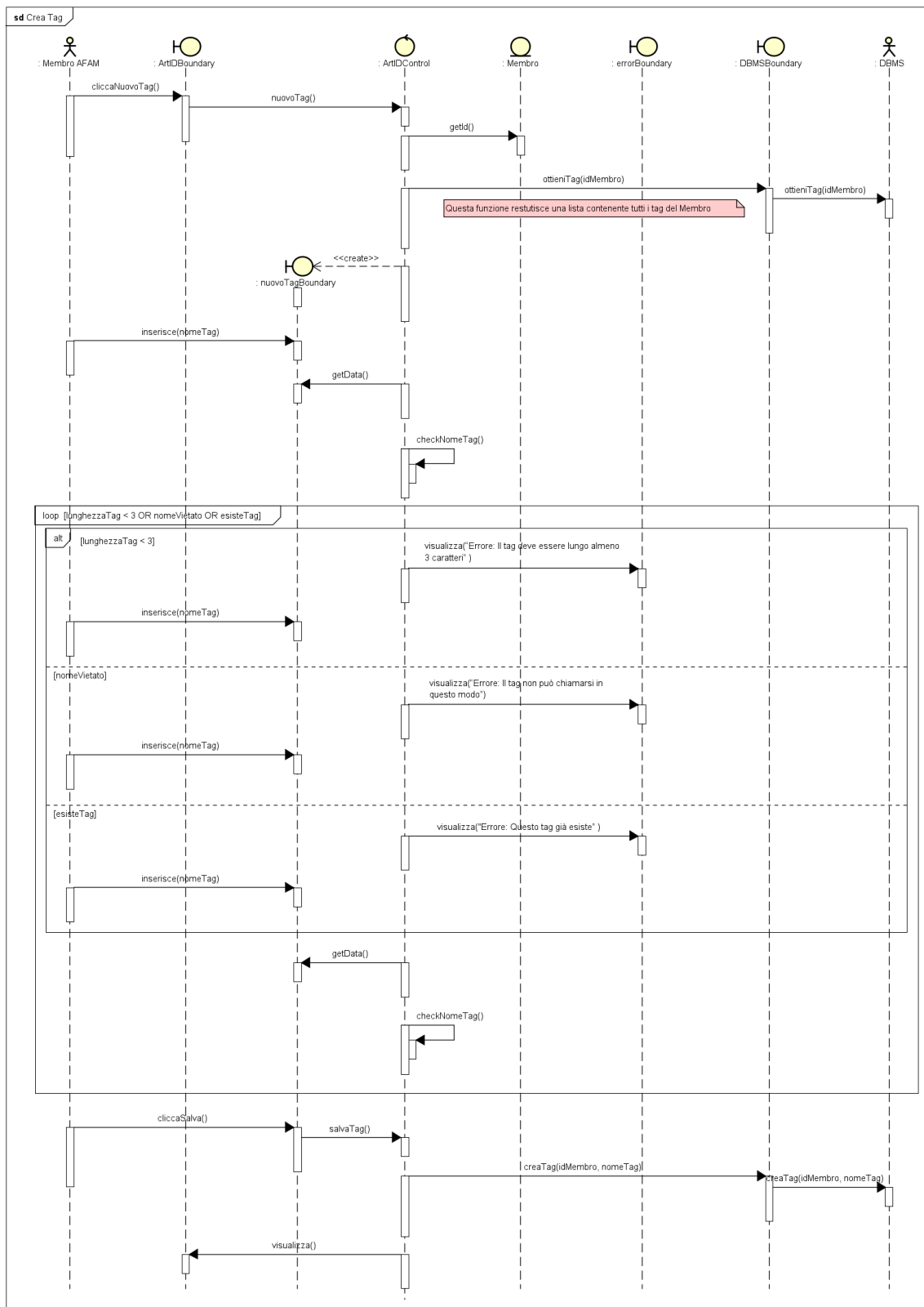
Figure 31: Crea Tag
