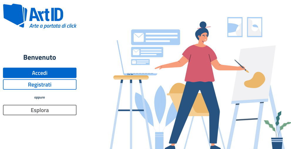
Figure 52: Schermata Welcome
