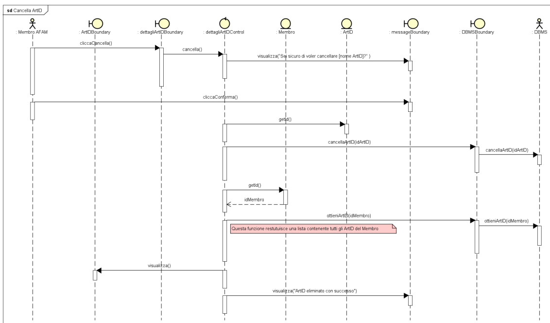
Figure 28: Cancella ArtID
