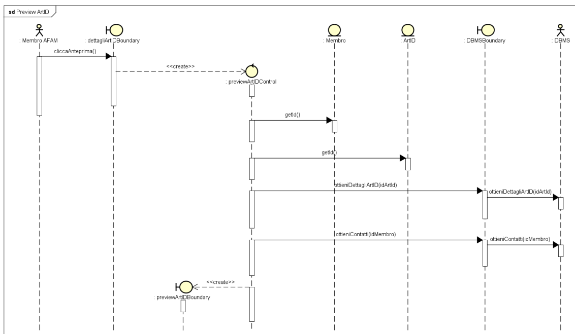
Figure 34: Preview ArtID
