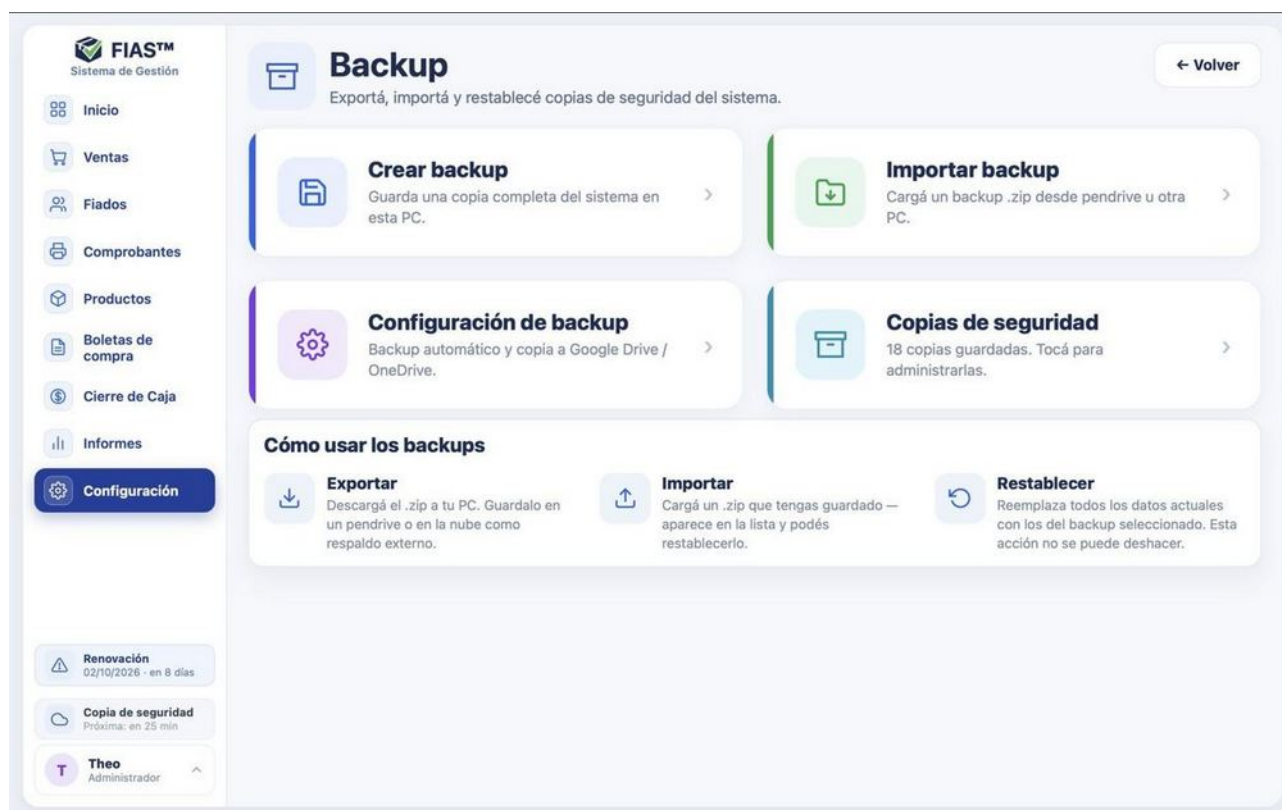
Figura 100 — Backup.
