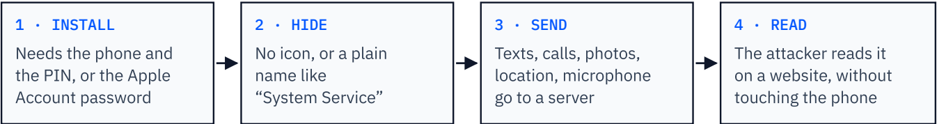
FIGURE 1 — HOW STALKERWARE WORKS
