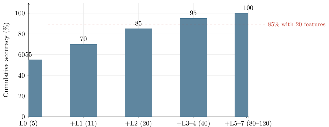
Figure 8.1: Cumulative accuracy by feature layer. Parentheses show total feature count at each stage. The dashed line marks the 85% threshold achievable with Layers 0–2 and a Ridge regression.
