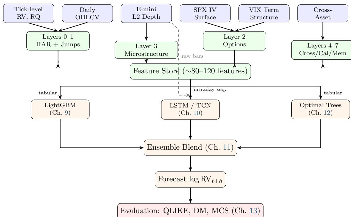
Figure 14.1: End-to-end pipeline from raw data to scored forecasts. Blue: data sources. Green: feature computation and storage. Orange: models and blending. Red: evaluation. Dashed arrow indicates the LSTM also receives raw intraday bar sequences directly.
