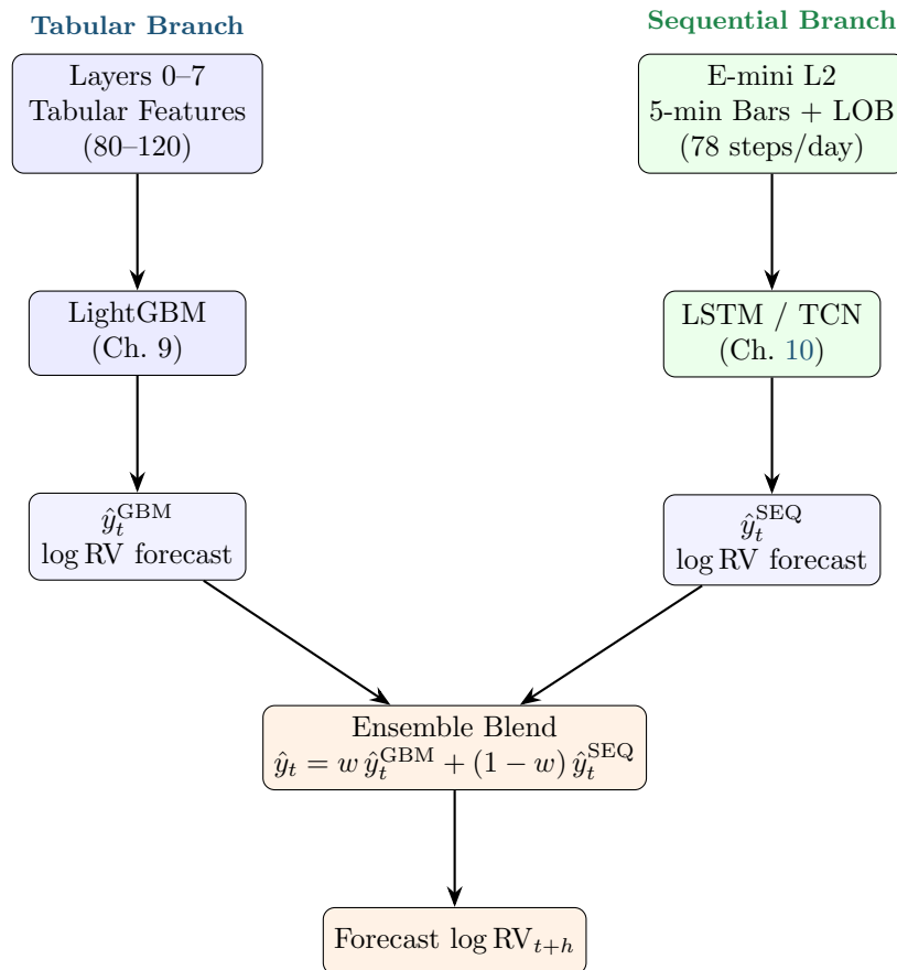
Figure 11.1: Two-branch ensemble architecture. Each branch independently forecasts \log \text{RV}_{t+h} ; outputs are blended at the prediction level.
