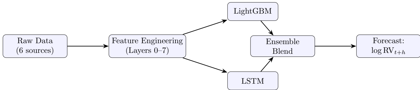
Figure 1.1: High-level forecasting pipeline.
