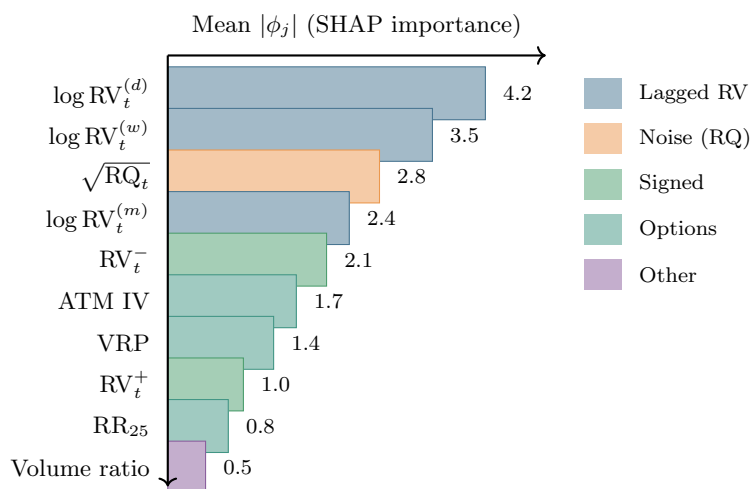
Figure 10.6: Illustrative SHAP feature importance ranking for a gradient-boosted tree model forecasting next-day log-RV. Lagged RV features (blue) dominate, but noise-awareness ( \sqrt{RQ_t} , orange) and asymmetry ( RV_t^- , green) provide substantial incremental value. Options-implied features (teal) add forward-looking information. Exact values are dataset-dependent; the ranking pattern is robust.
