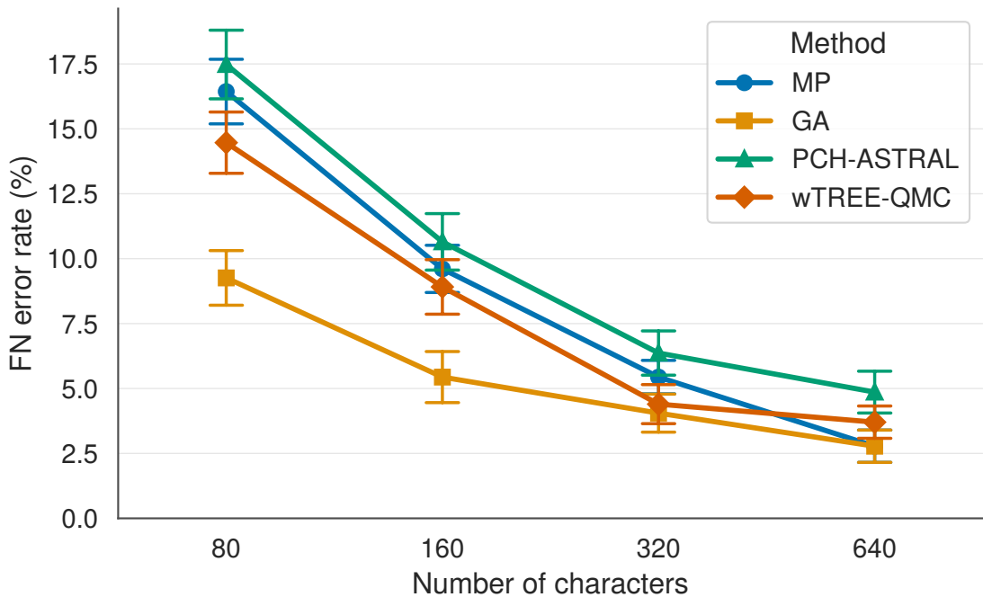
FN error vs number of characters
