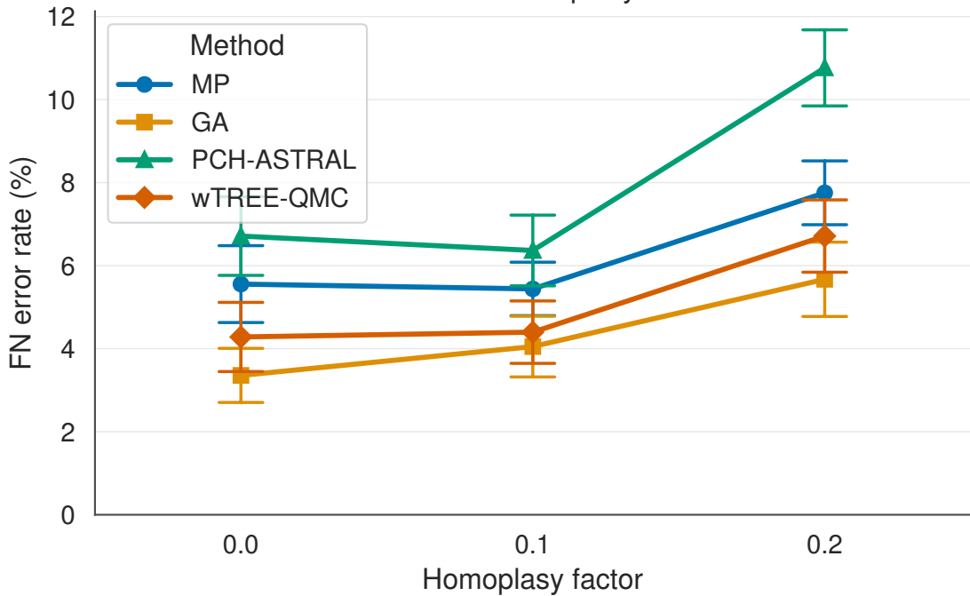
FN error vs homoplasy factor
