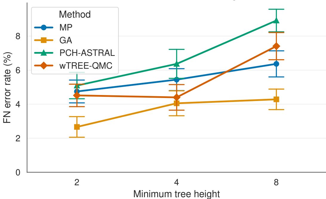
FN error vs minimum tree height
